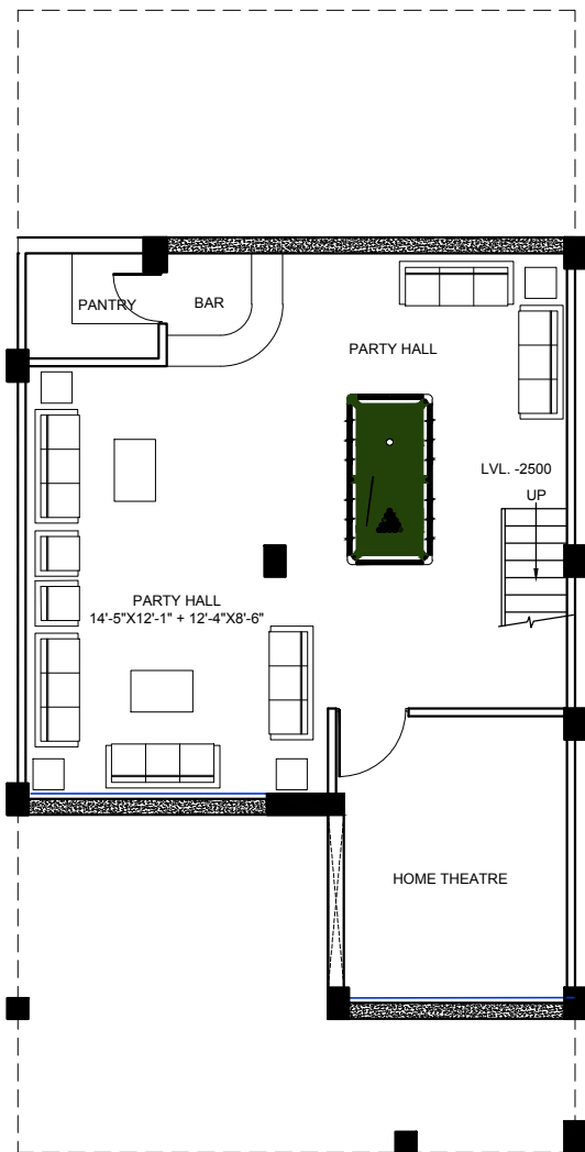
BASEMENT PLAN
