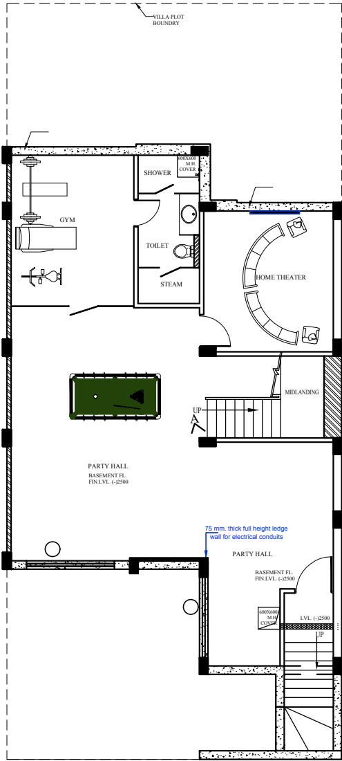
BASEMENT PLAN
