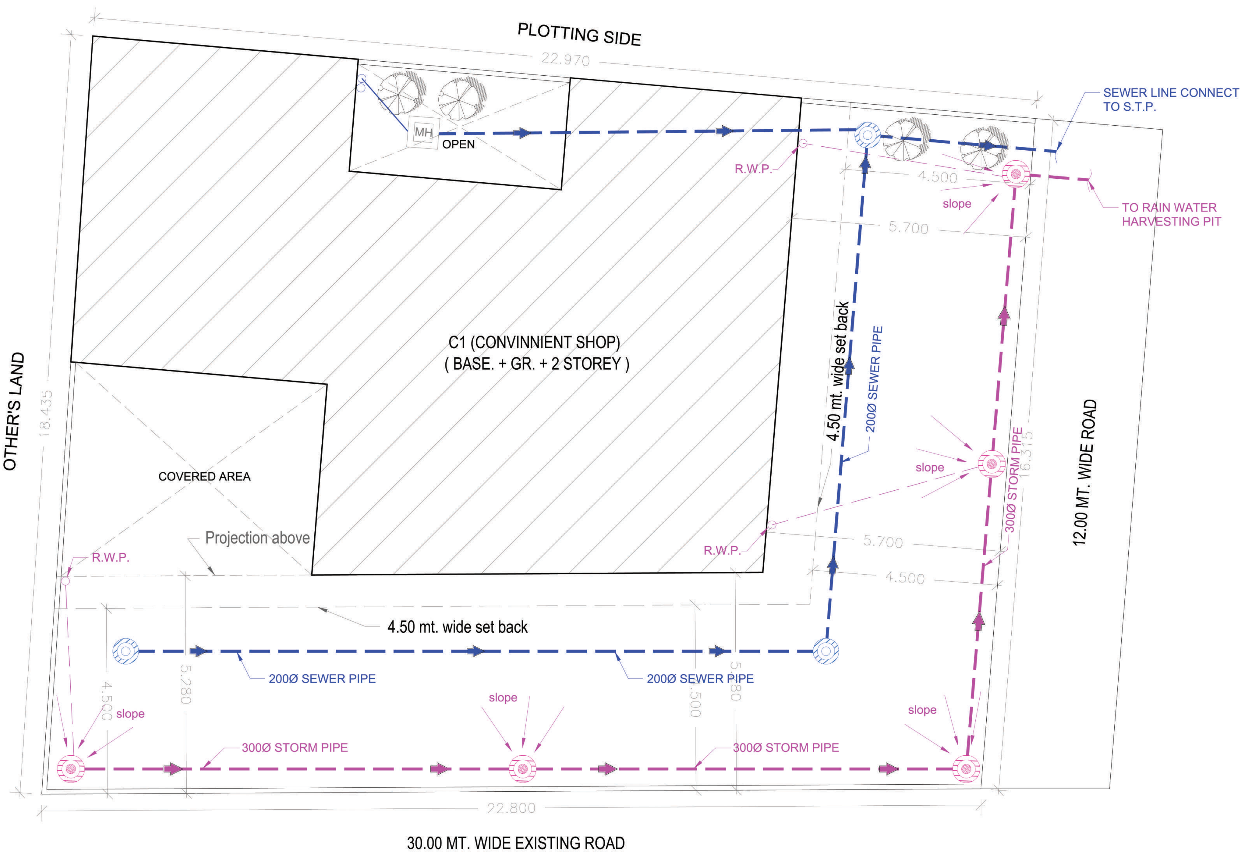
STROM WATER & SEWAGE PLAN
