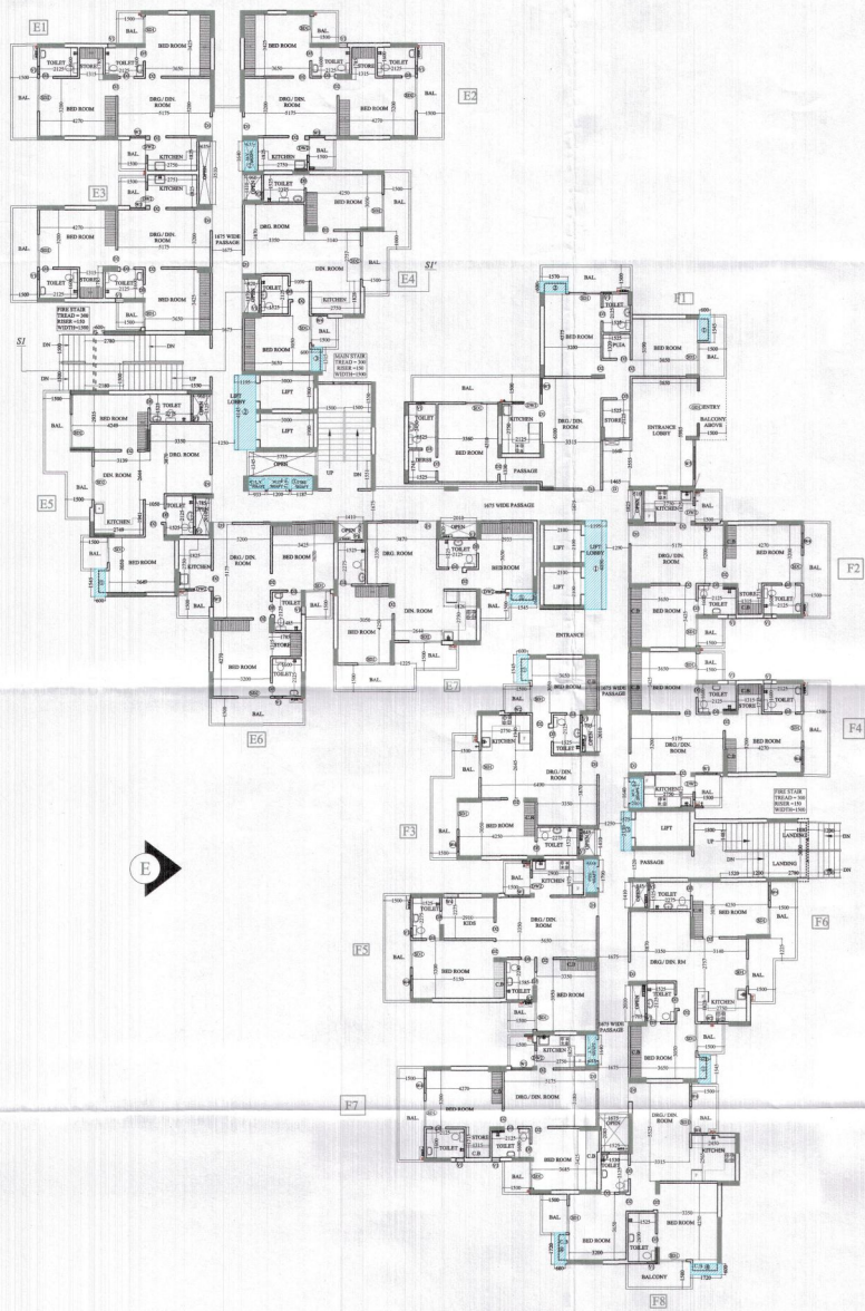
TOWER - E & F GROUND FLOOR PLAN
