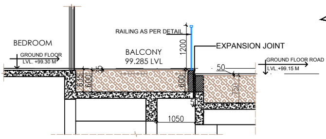
SECTION 2-2 THROUGH BEDROOM & BALCONY
