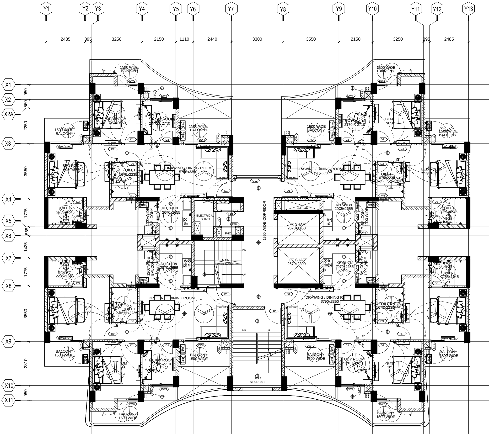
9TH TO 19TH FLOOR PLAN
