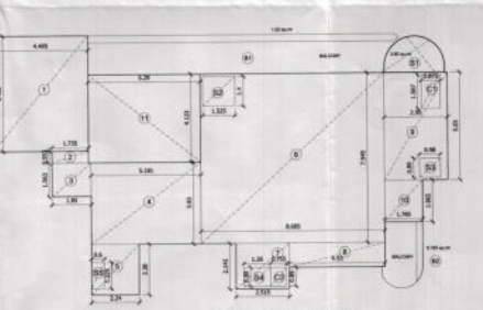
FIRST FLOOR F.A.R AREA CALCULATION CHART TYPE-II 3BHK
