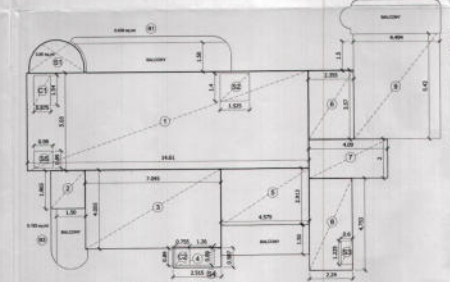
FIRST FLOOR F.A.R AREA CALCULATION CHART TYPE-I 3BHK
