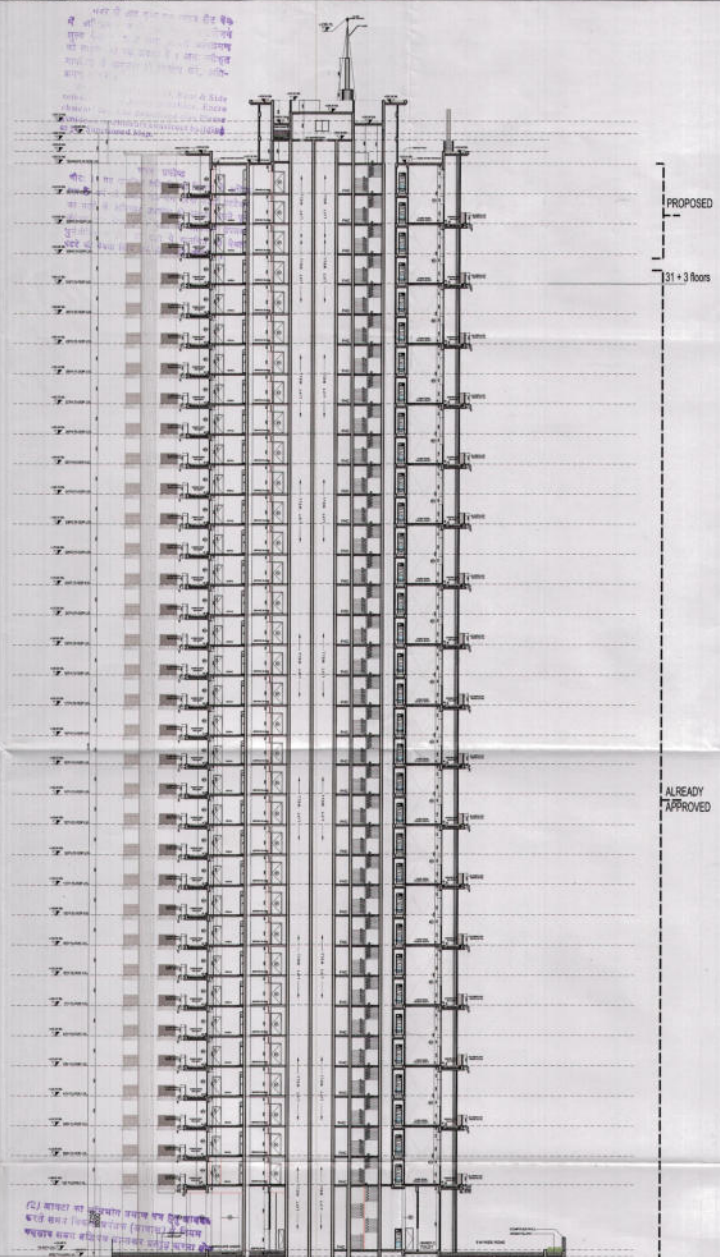
4BHK STAGGERED SECTION A-A
