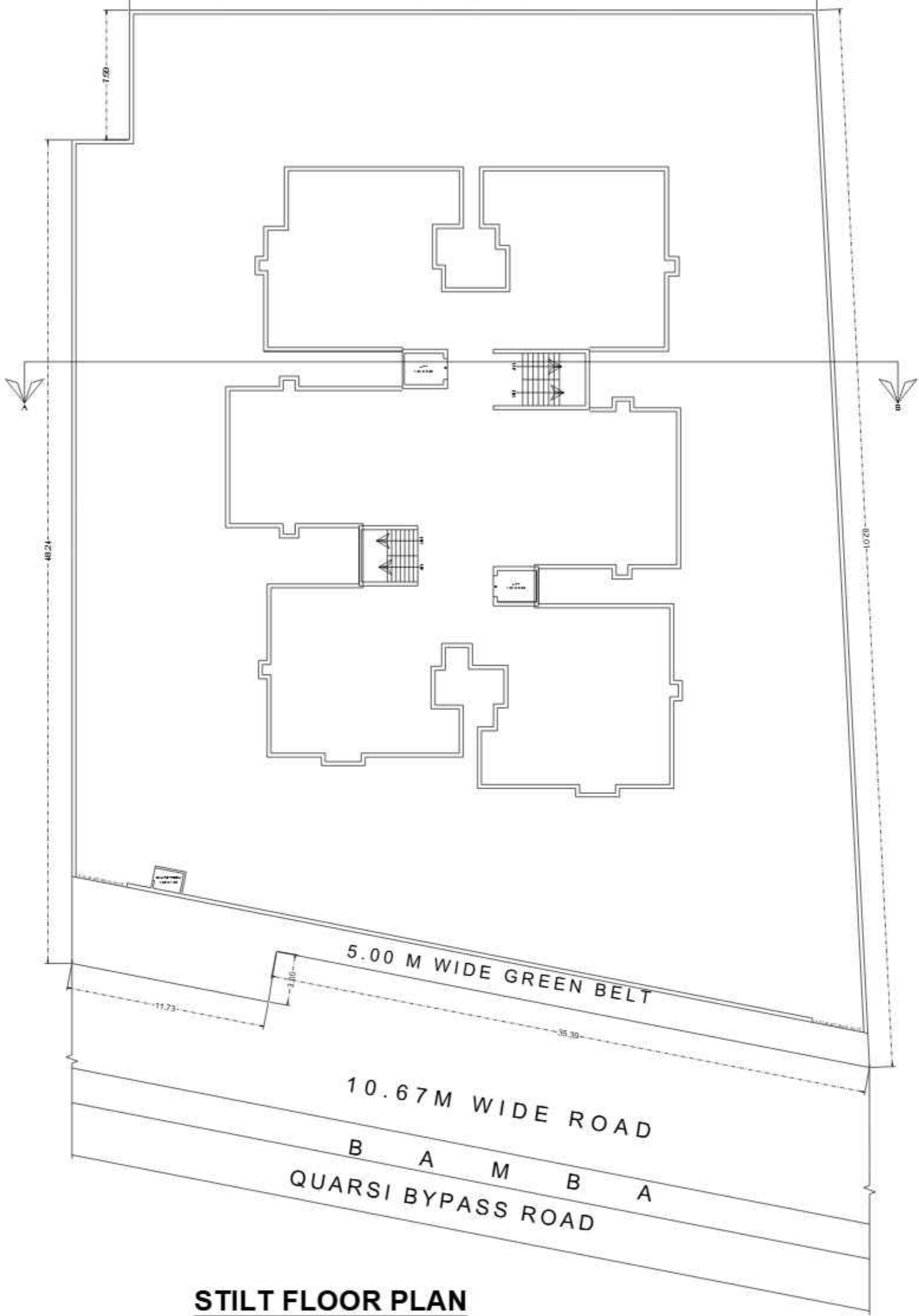
STILT FLOOR PLAN
