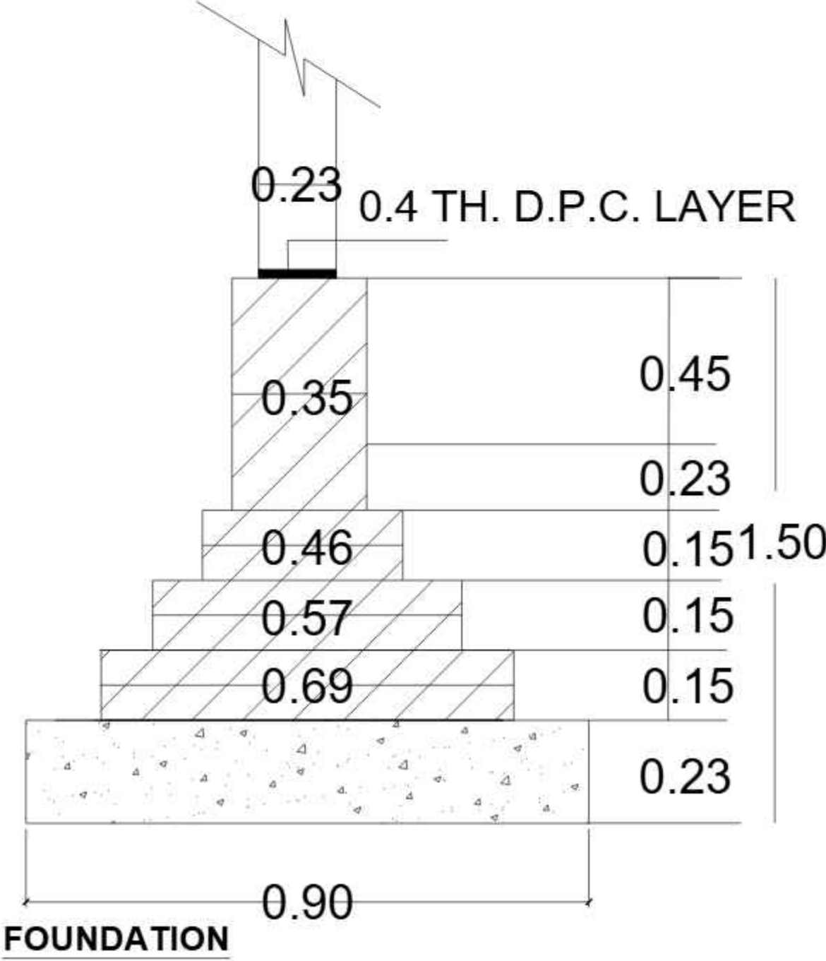
FOUNDATION
