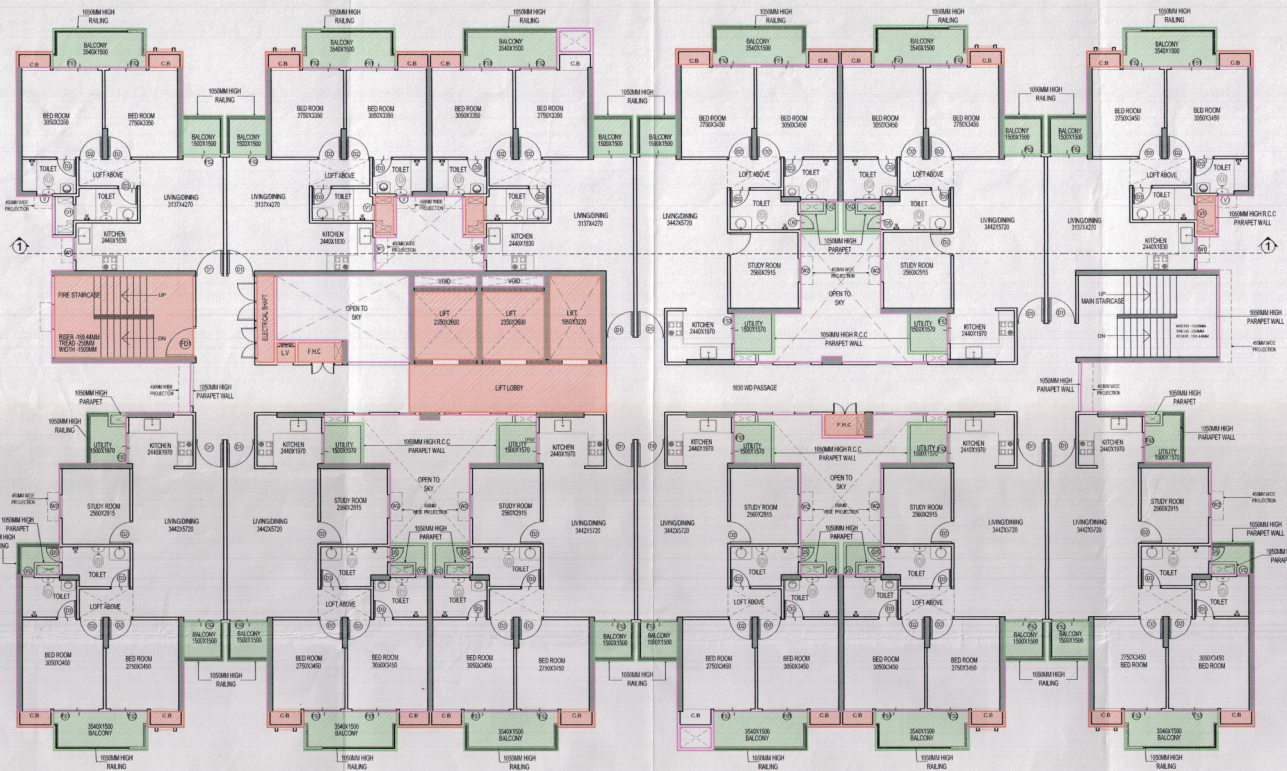
GREEN SIDE TYPICAL FLOOR PLAN TYPE-2
