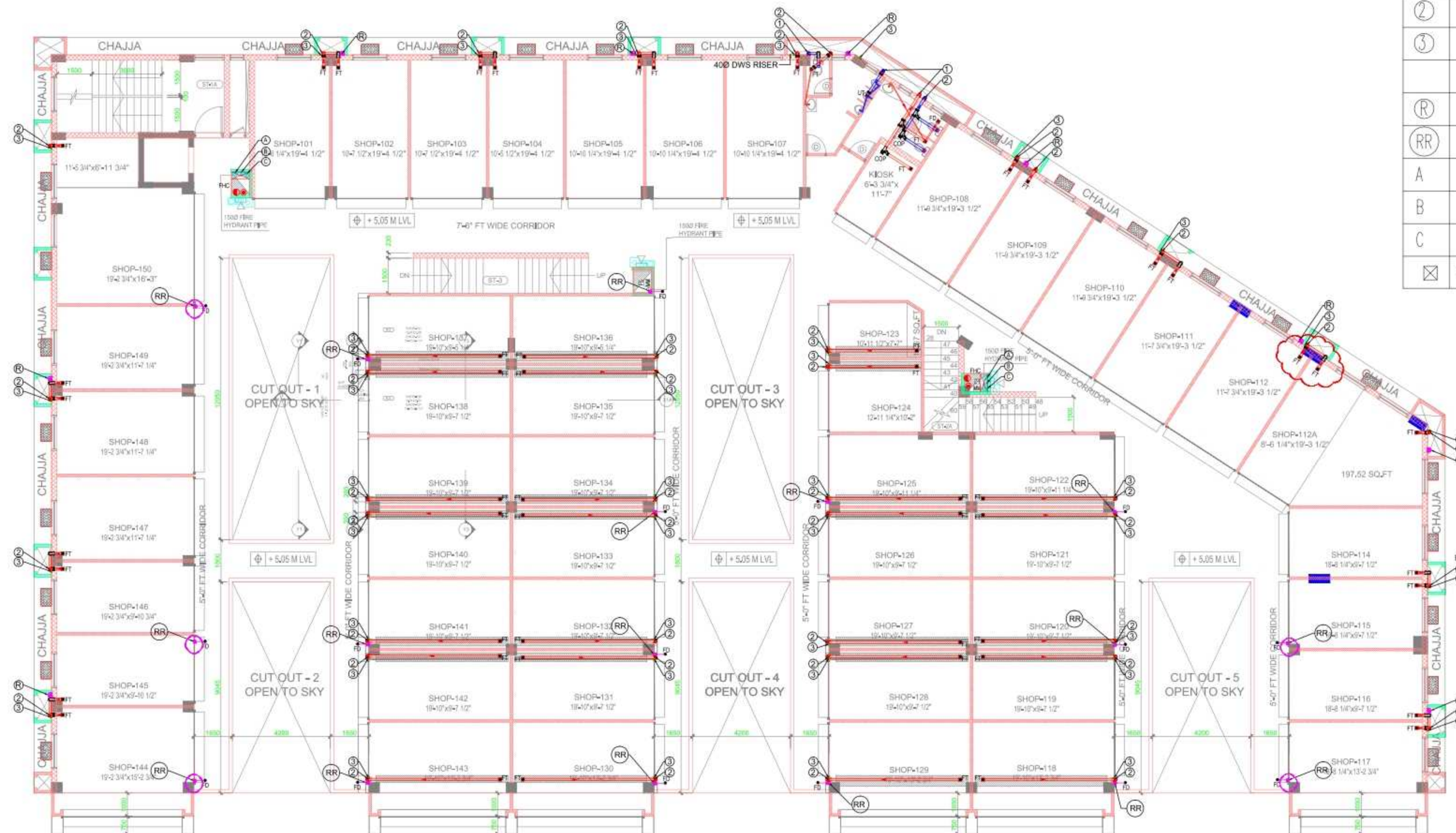
1ST FLOOR PLUMBING LAYOUT
