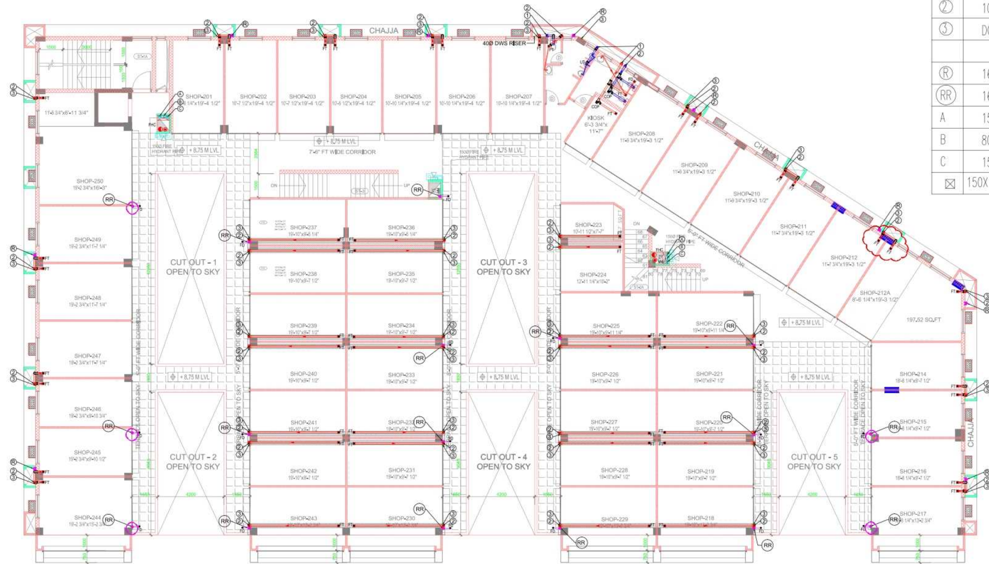
2ND FLOOR PLUMBING LAYOUT
