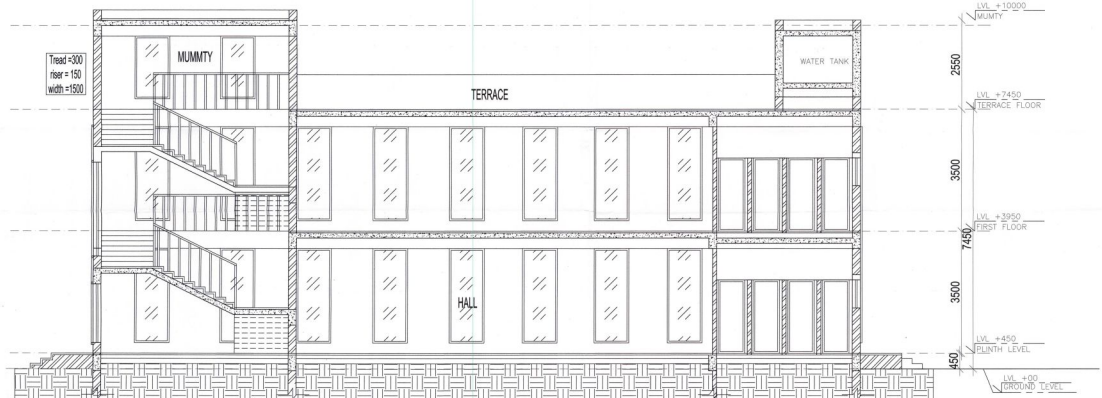
SECTION BB SCALE=1:50
