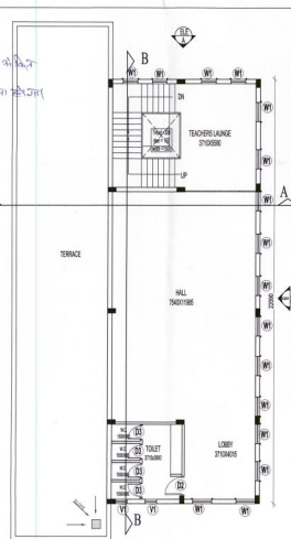
1ST FLOOR PLAN SCALE=1:100
