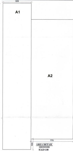
GROUND FLOOR PLAN SCALE=1:100
