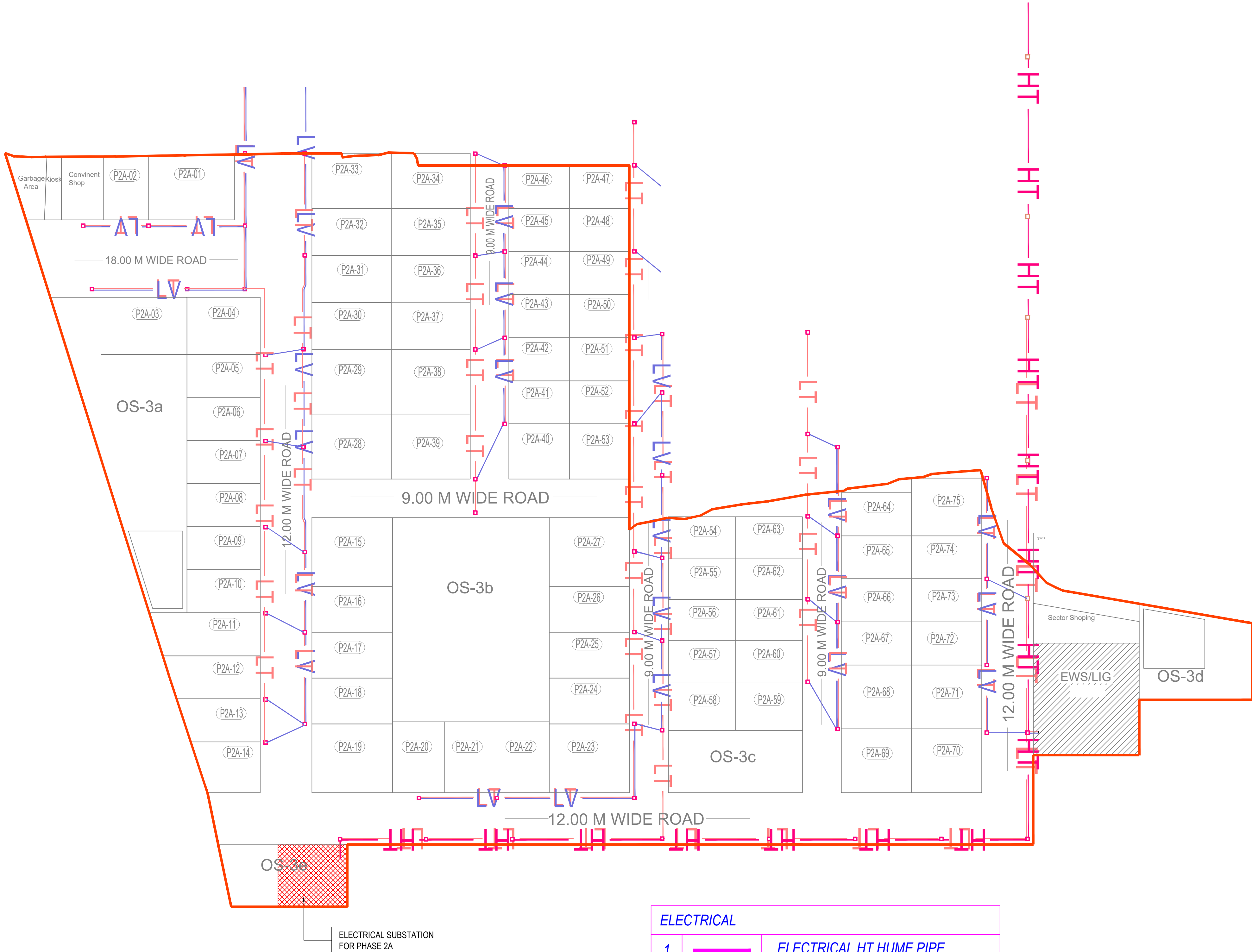
ELECTRICITY PLAN
