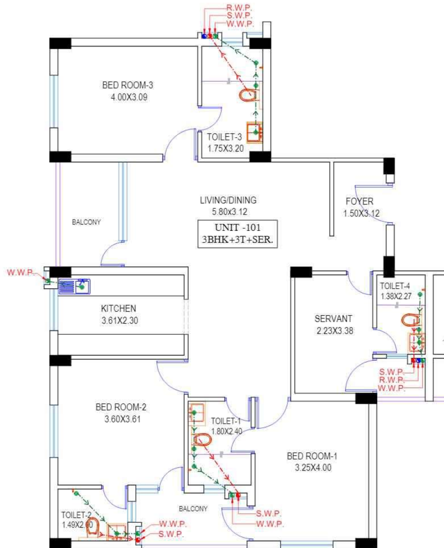
TOWER 1B (UNIT -101, 3BHK+3T+SER.)
