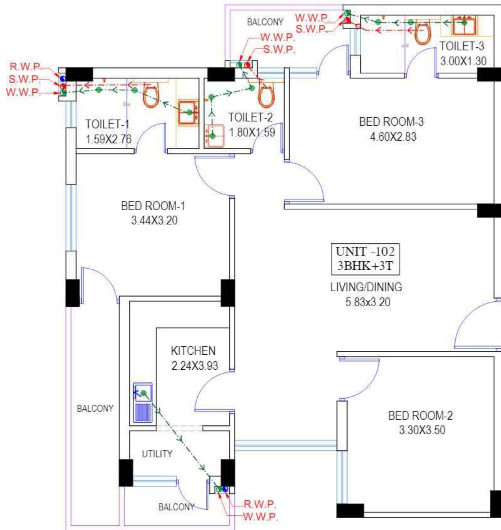
TOWER 1B (UNIT -102, 3BHK+3T)
