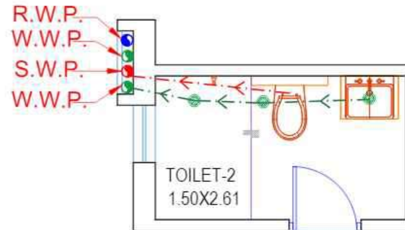
TOILET.-2 (UNIT-103)
