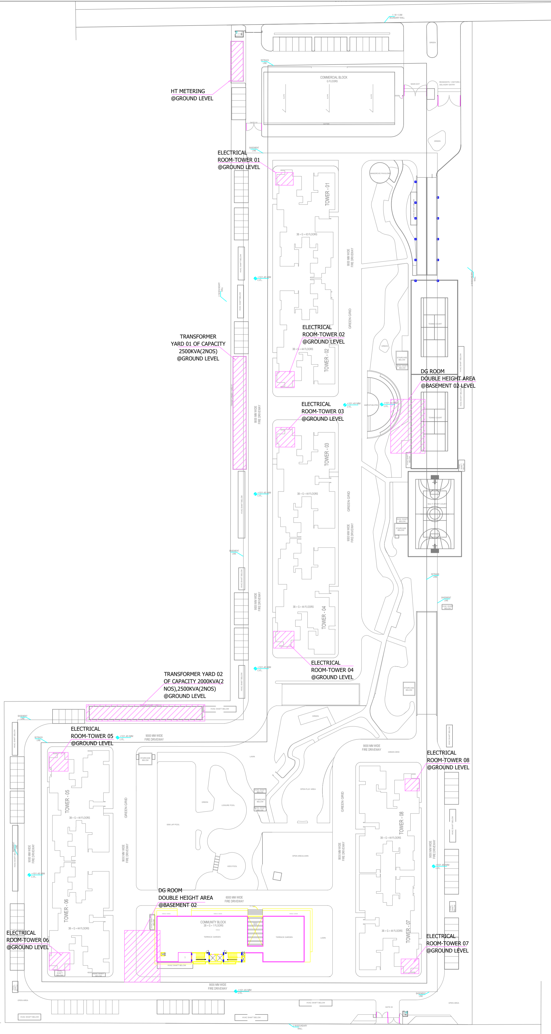
KEY PLAN
