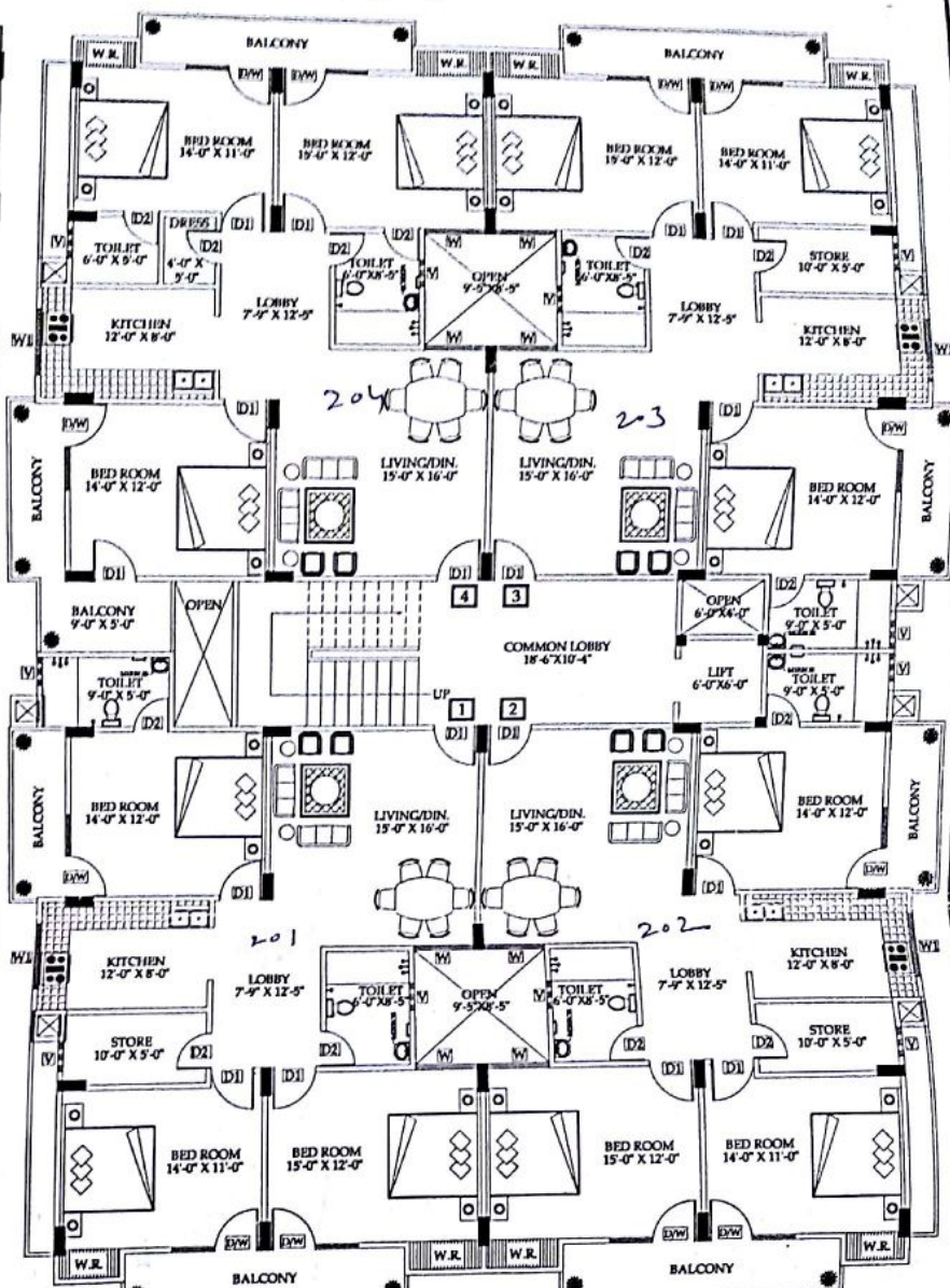
TYPICAL FLOOR PLAN SCALE :- 1" = 8'-0"
