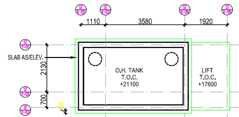
OH TANK TERRACE PLAN
