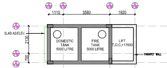
OVERHEAD TANK PLAN
