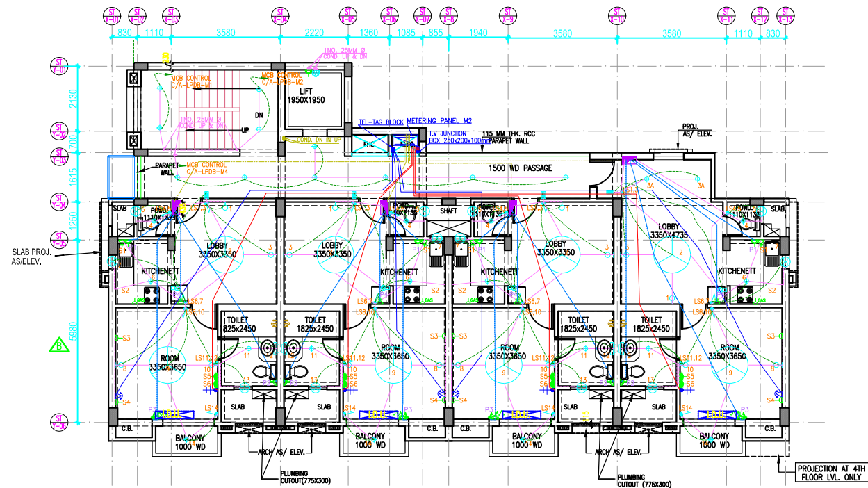
TYPICAL FLOOR PLAN (2ND TO 4TH FLOOR)
