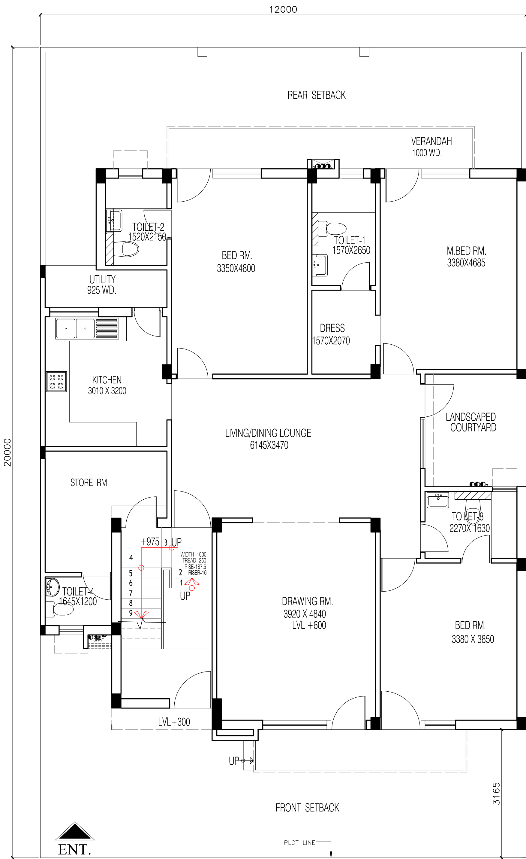
WAVE / PRIME FLOOR (240sqm) SITE PLAN
