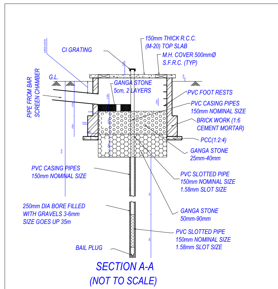
Rain Water Harvesting Details
