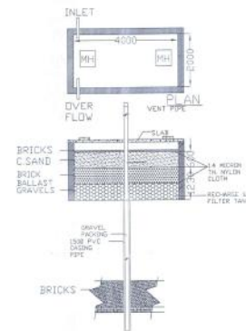
X-SECTION DETAIL OF R.W.H.PIT & WELL (NTS)
