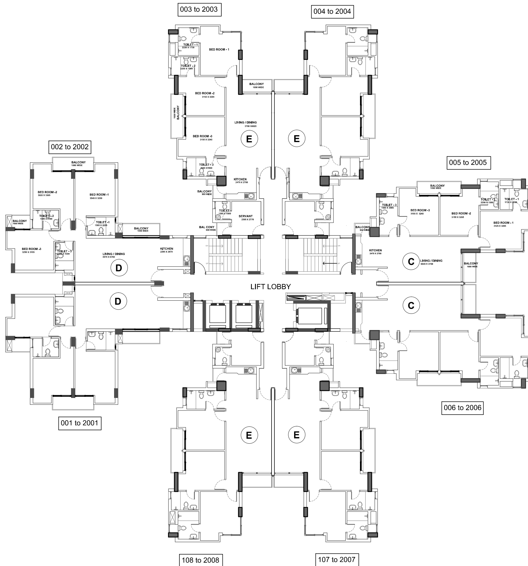
TYPICAL FLOOR PLAN - 3BHK
