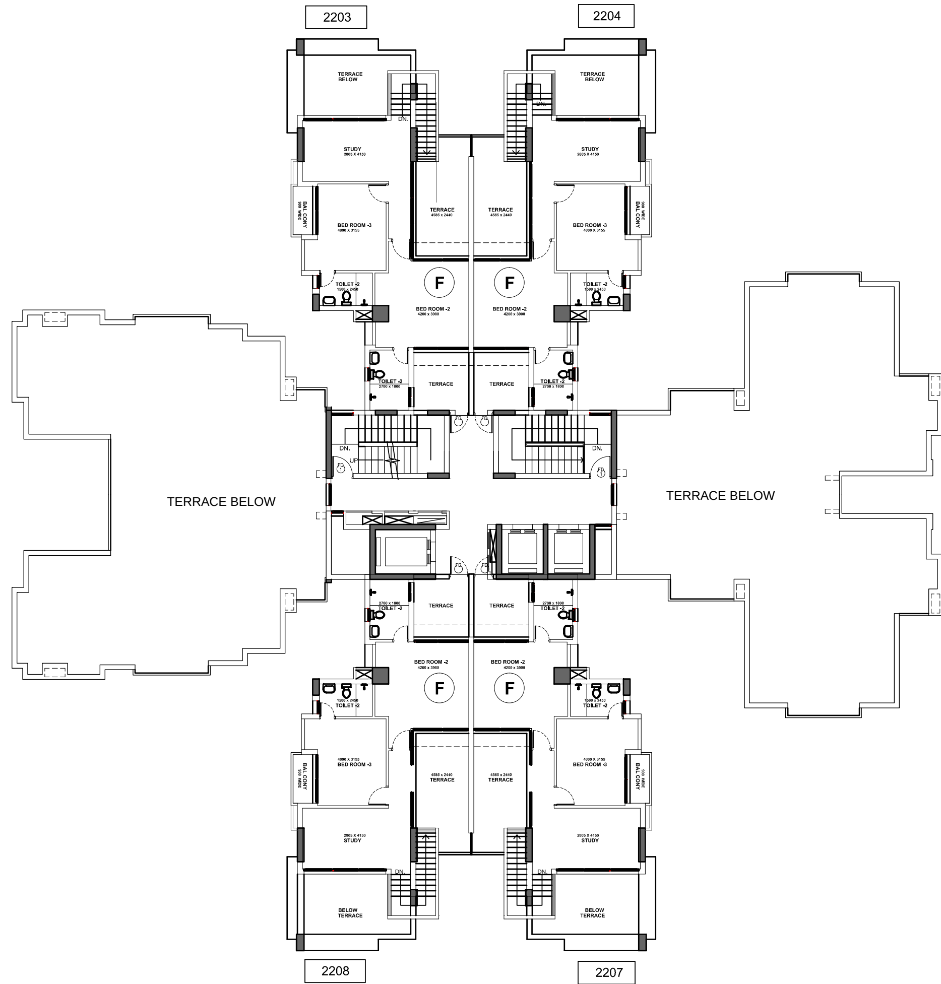
TYPICAL FLOOR PLAN - DUPLEX 3BHK (UPPER LEVEL PLAN)
