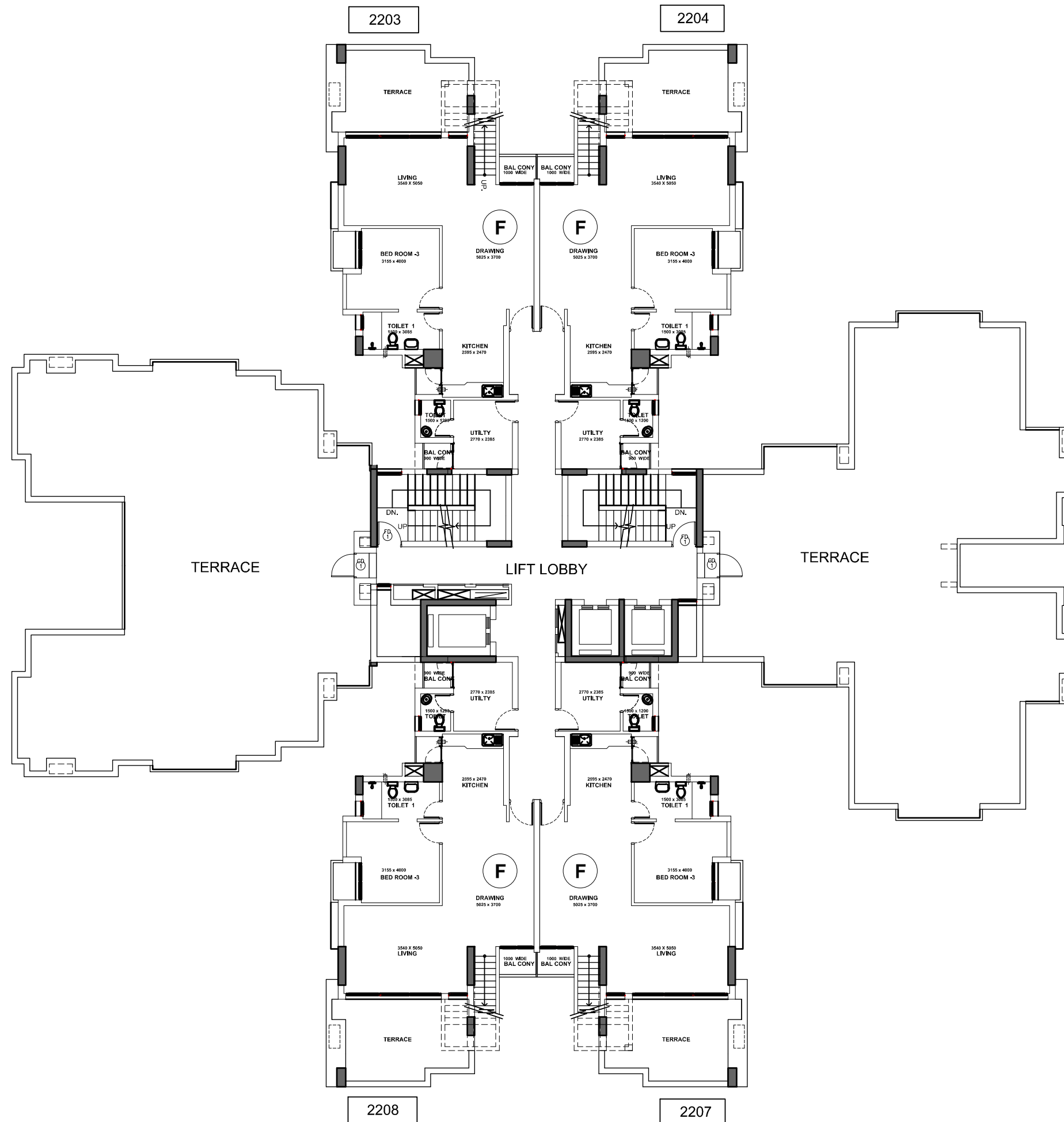
TYPICAL FLOOR PLAN - DUPLEX 3BHK (LOWER LEVEL PLAN)
