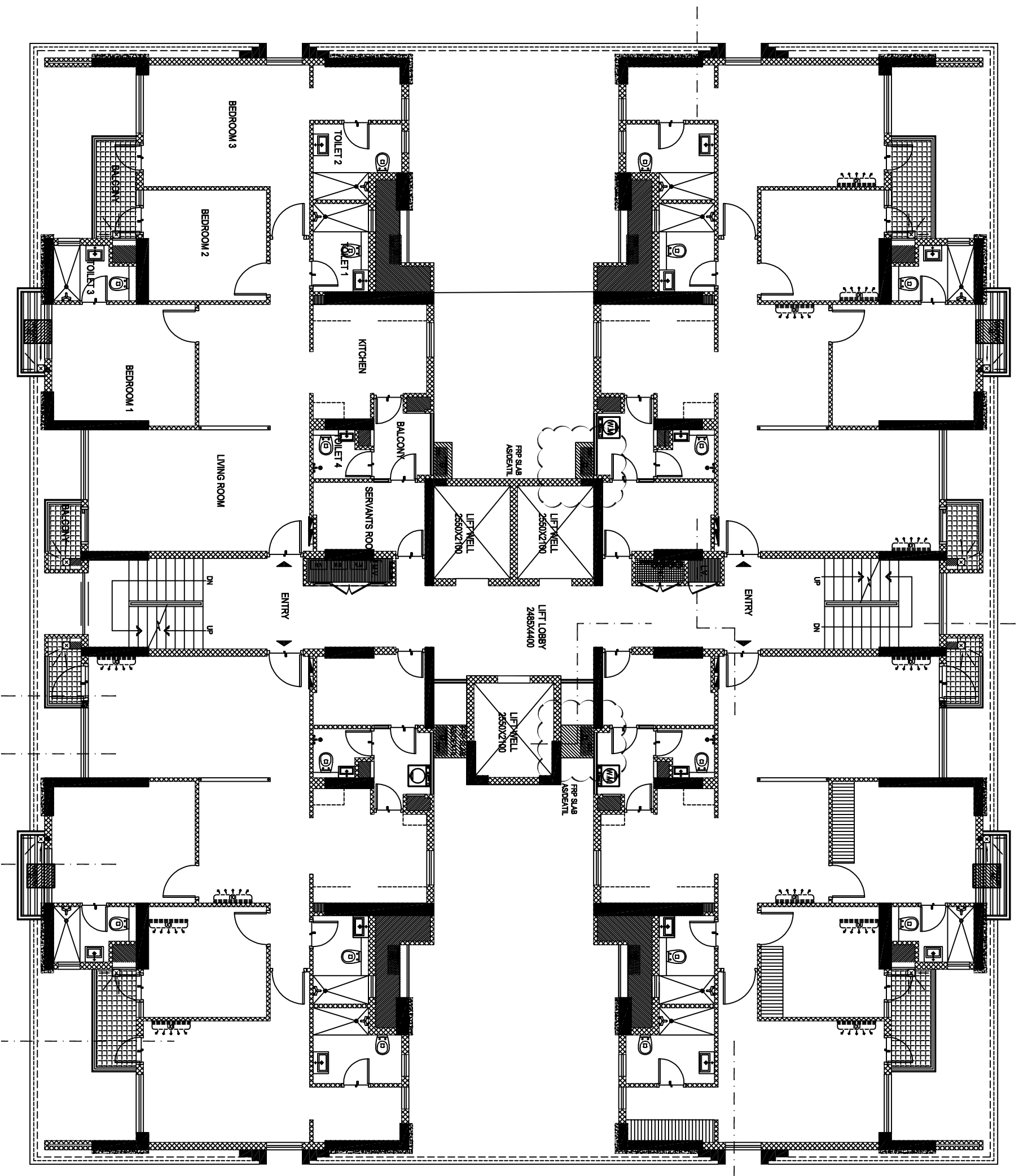
TYPICAL PLAN KSI-10,KSI-11(3BHK)
