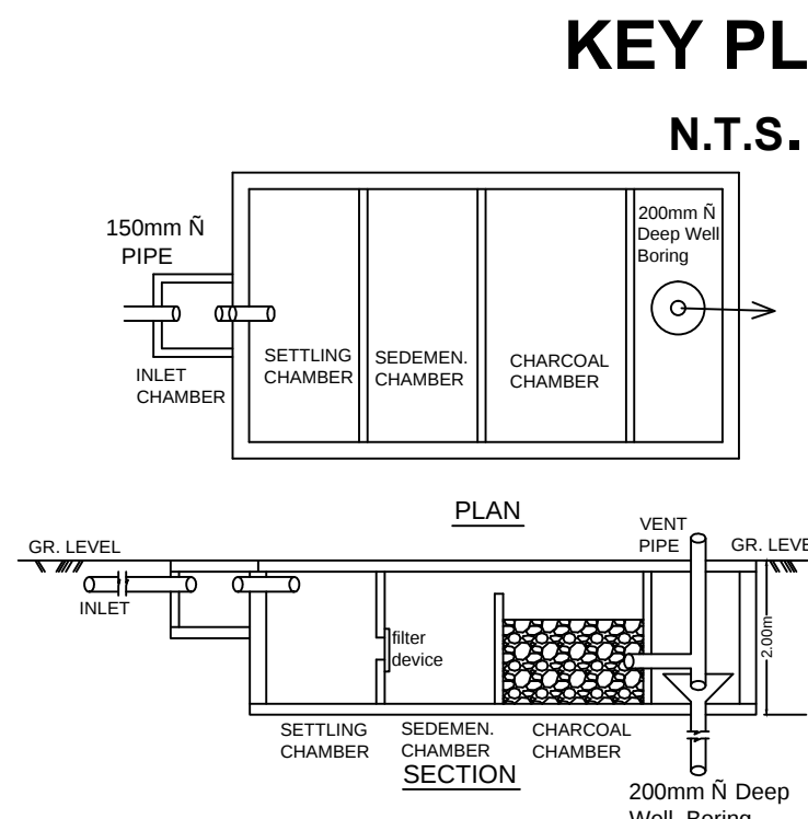
DETAIL OF RAIN WATER HARVESTING SYSTEM (NOT TO SCALE)
