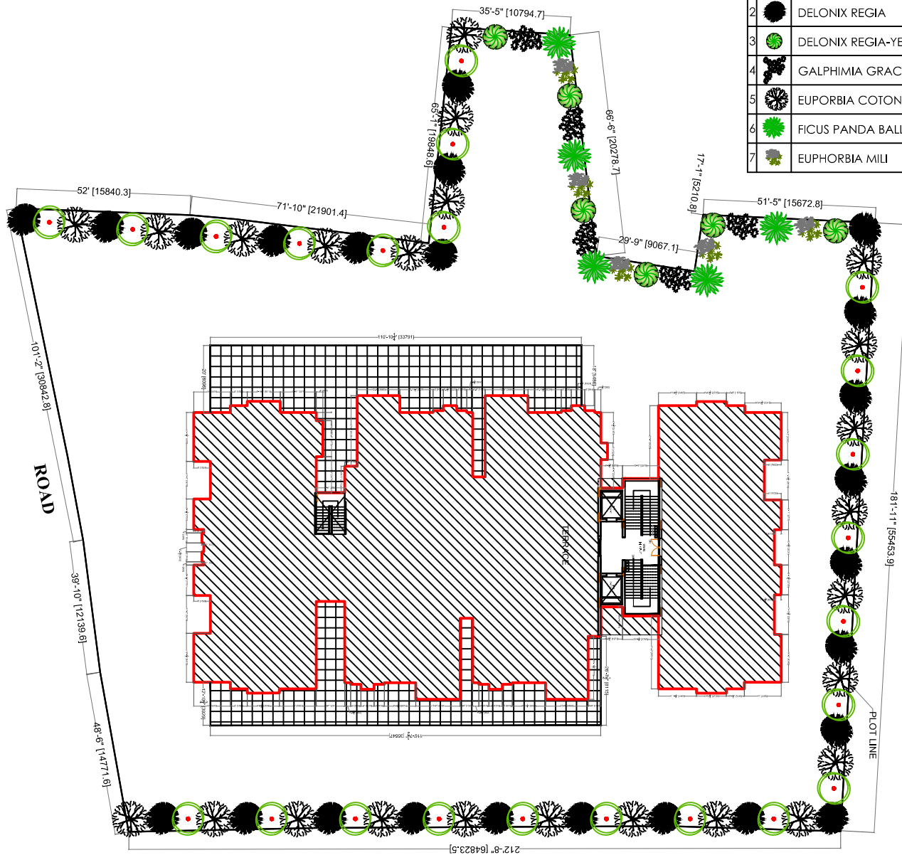
LANDSCAPE PLAN
