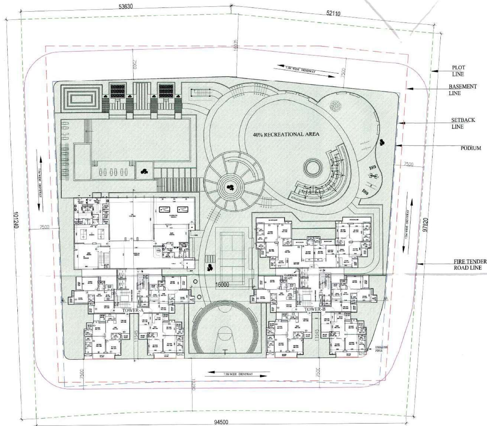
LANDSCAPE PLAN
