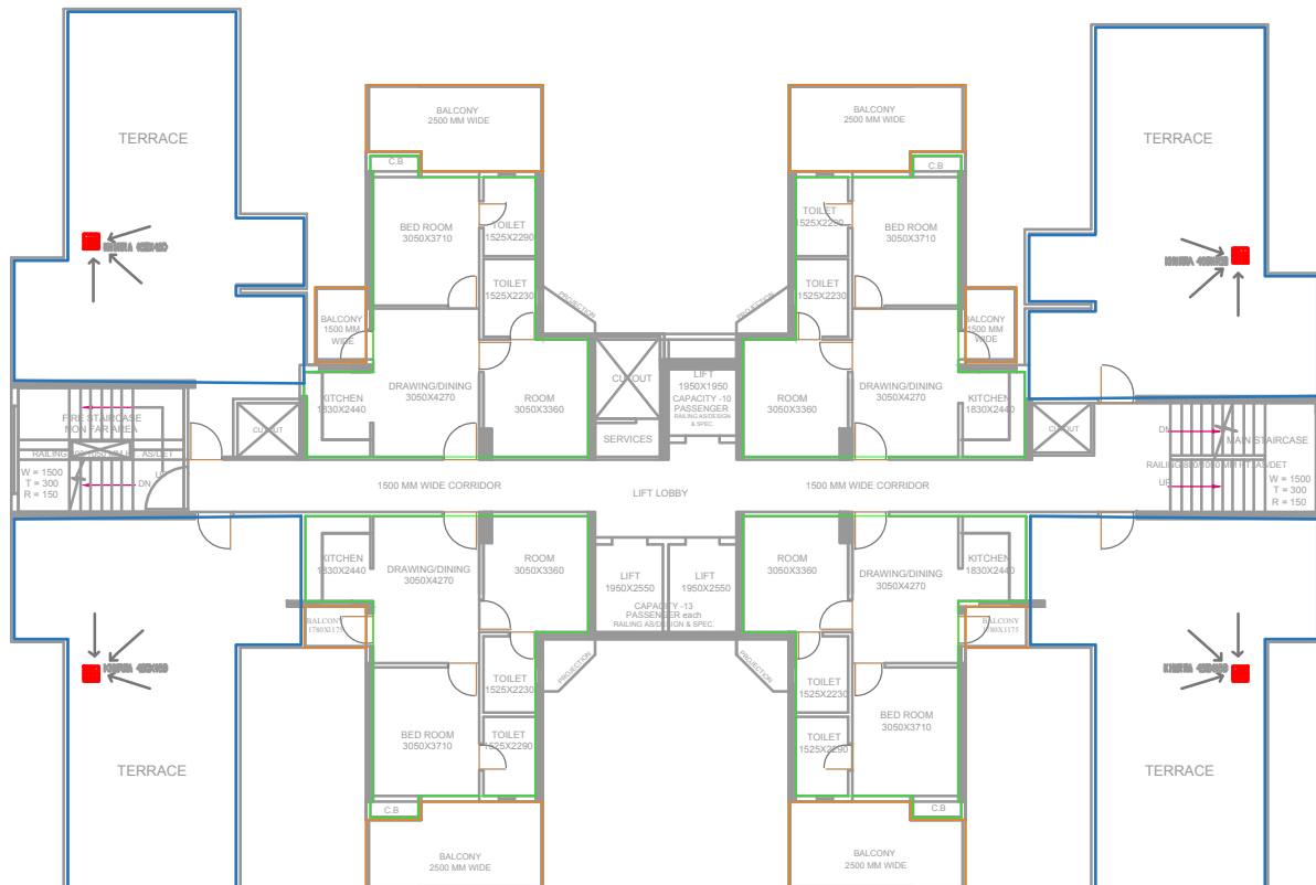
32nd FLOOR PLAN ( BLOCK-I)
