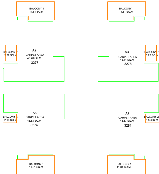
32nd FLOOR PLAN ( BLOCK-I)
