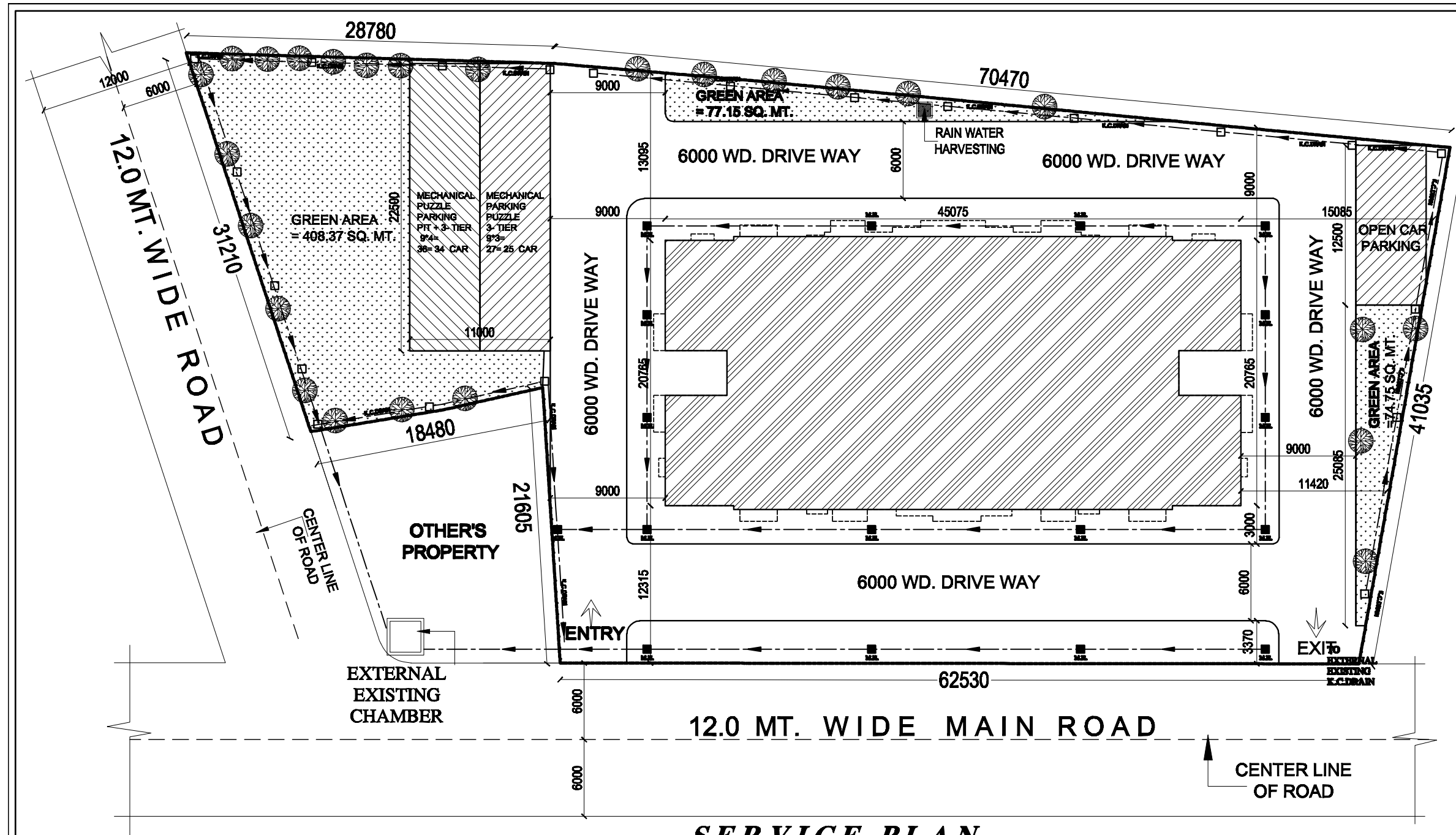
SERVICE PLAN (SCALE 1:100)
