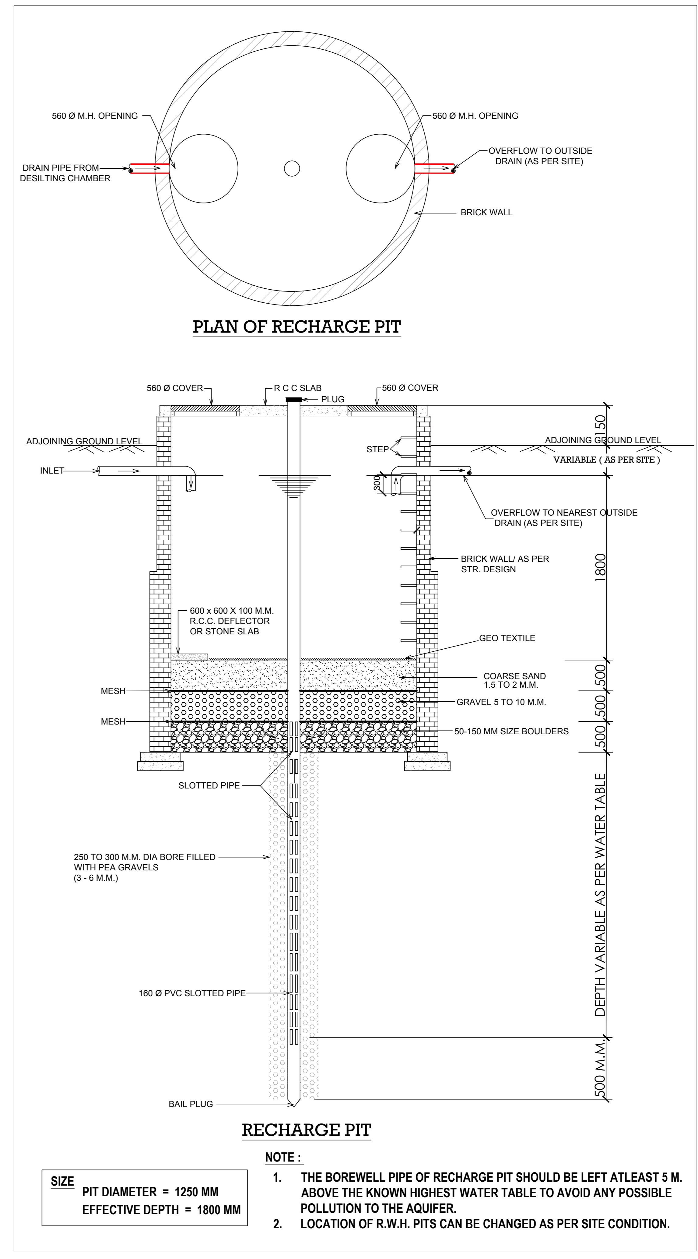
DRAINAGE /RAIN WATER HARVESTING LAYOUT
