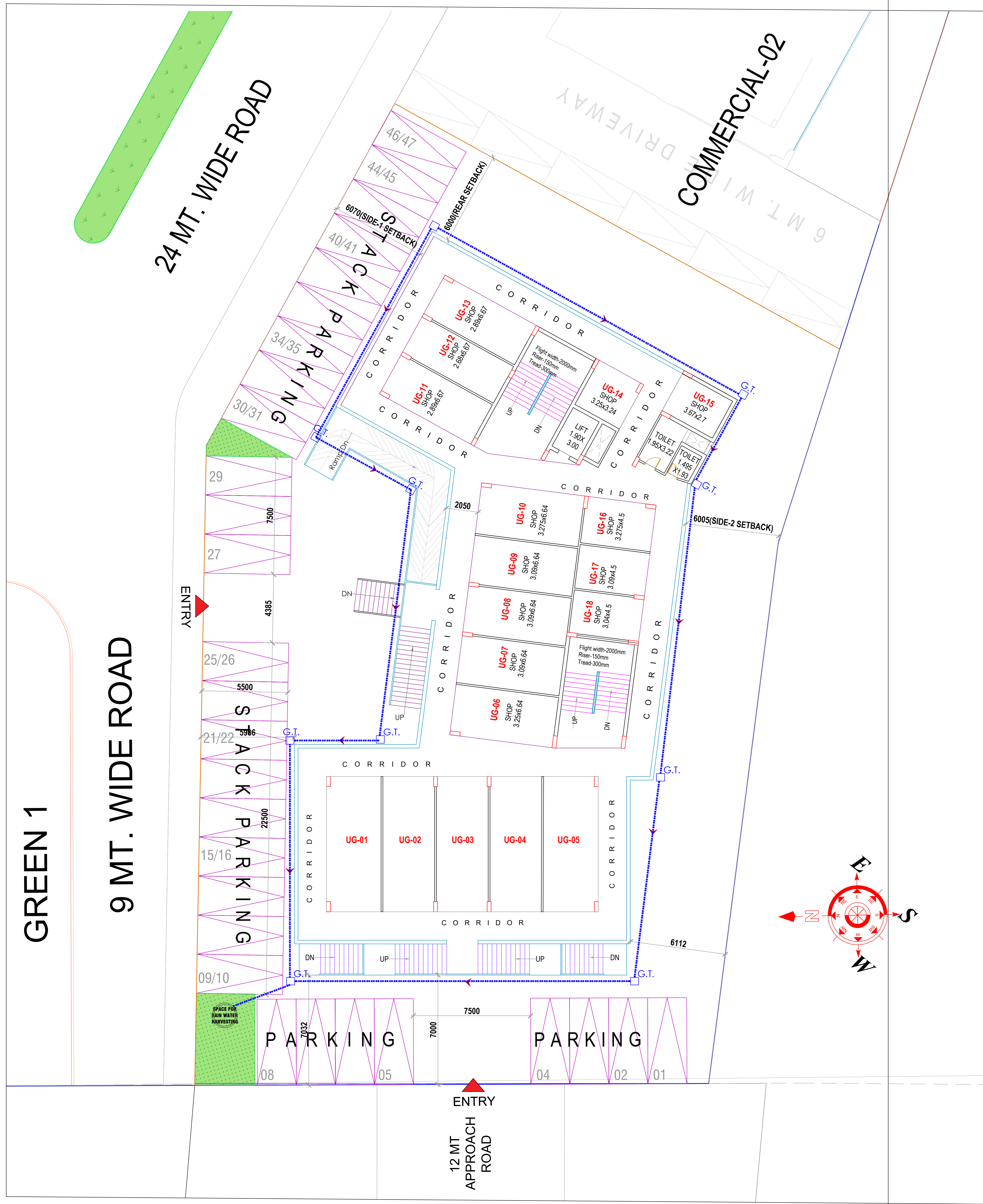
DRAINAGE /RAIN WATER HARVESTING LAYOUT SCALE=1:200
