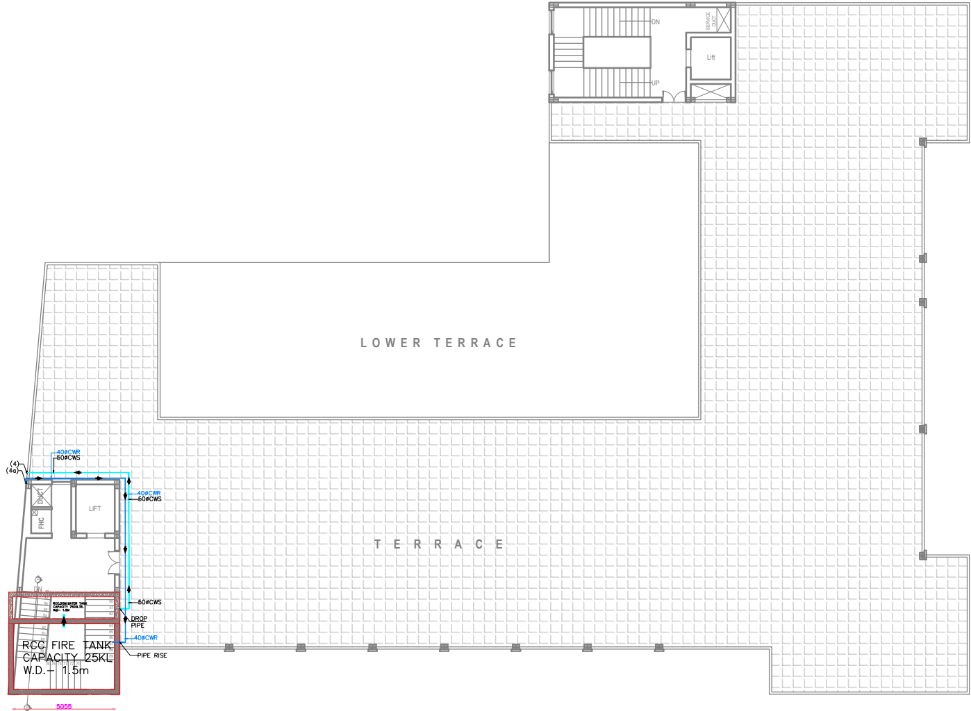
WATER SUPPLY TERRACE FLOOR PLAN
