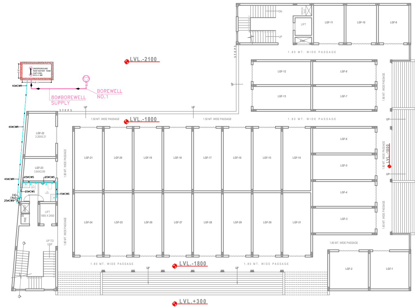
WATER SUPPLY LOWER GROUND FLOOR PLAN
