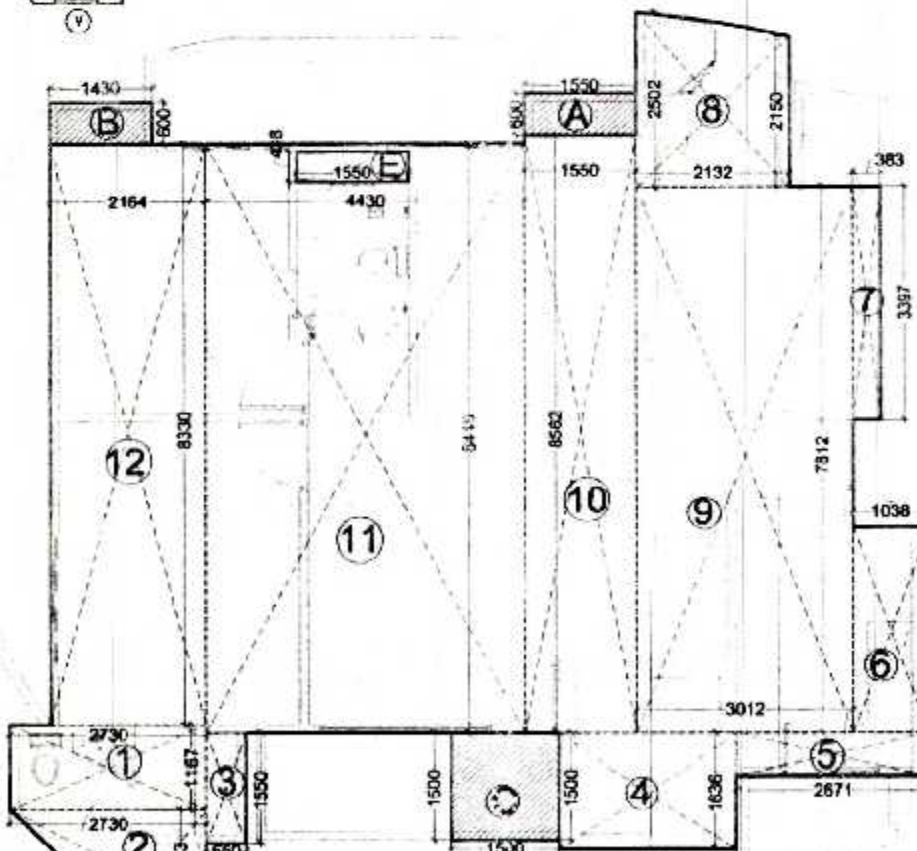
ENVELOP PLAN OF (TYPE-2)
