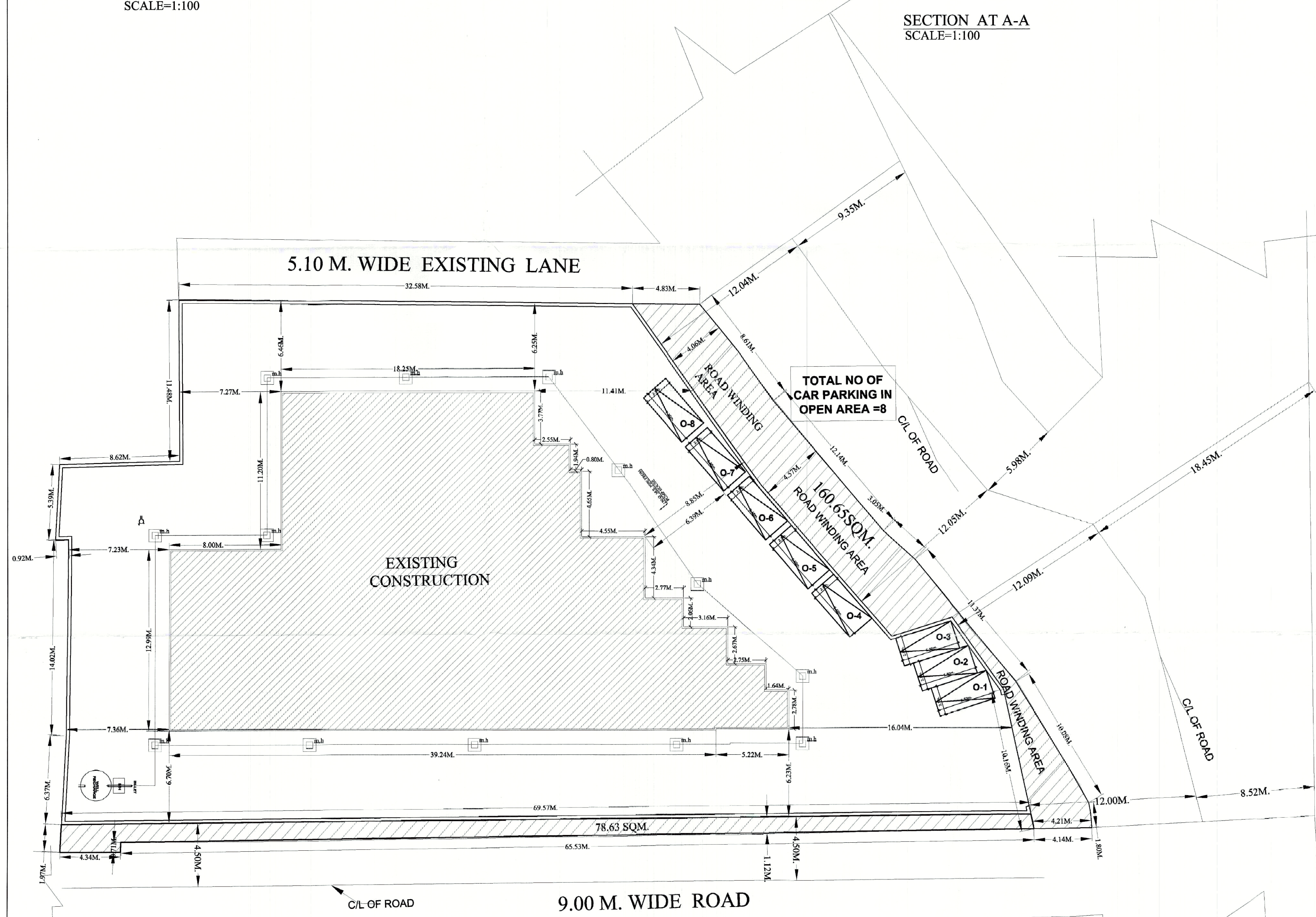
SITE PLAN
