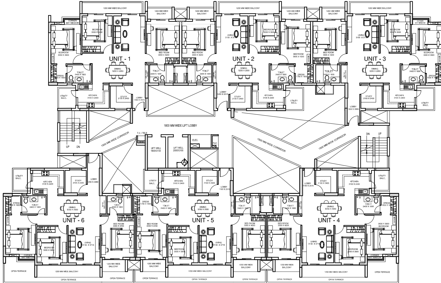
SECOND FLOOR -TOWER "A"
