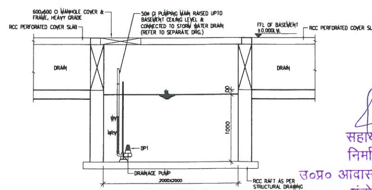
SECTION B-B (SCALE = NTS) (TYPICAL SECTION OF DRAINAGE SUMP DS1)
