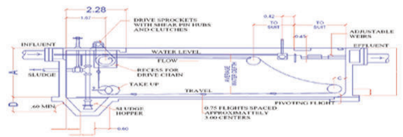
STP TANK DETAIL SCALE-N.T.S.
