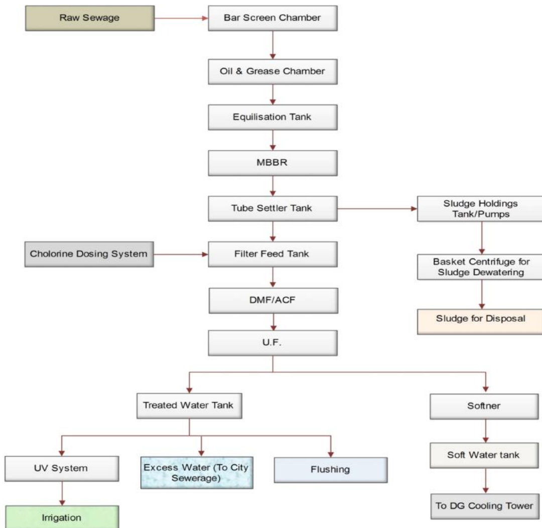
Figure 3: STP Process Flow Diagram
