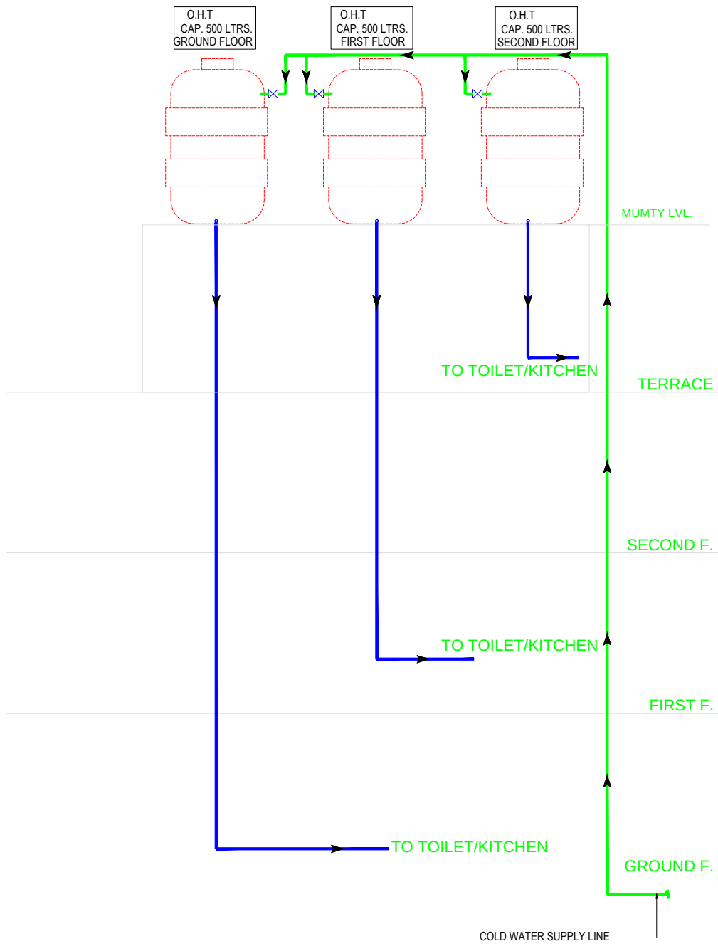
TYPICAL WATER SUPPLY SLD FOR FLOORS- WAVE FLOORS
