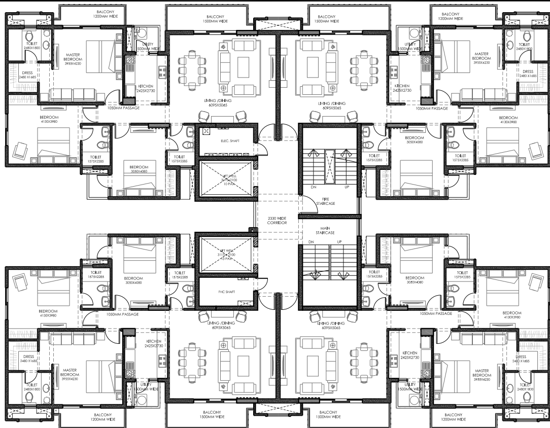
TYPICAL FLOOR PLAN, TYPE C; 3BHK+3T (TOWER-9, 10, 11)
