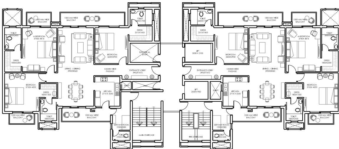
TYPICAL FLOOR PLAN, TYPE A2; 3BHK+UTILITY (TOWER-8)
