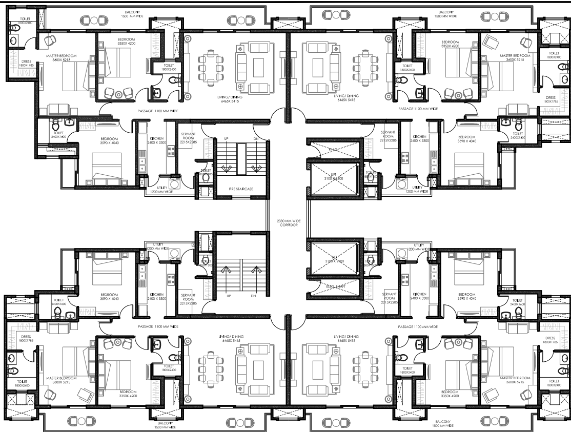
TYPICAL FLOOR PLAN, TYPE B; 3BHK+UTILITY (TOWER-4, 5, 6)
