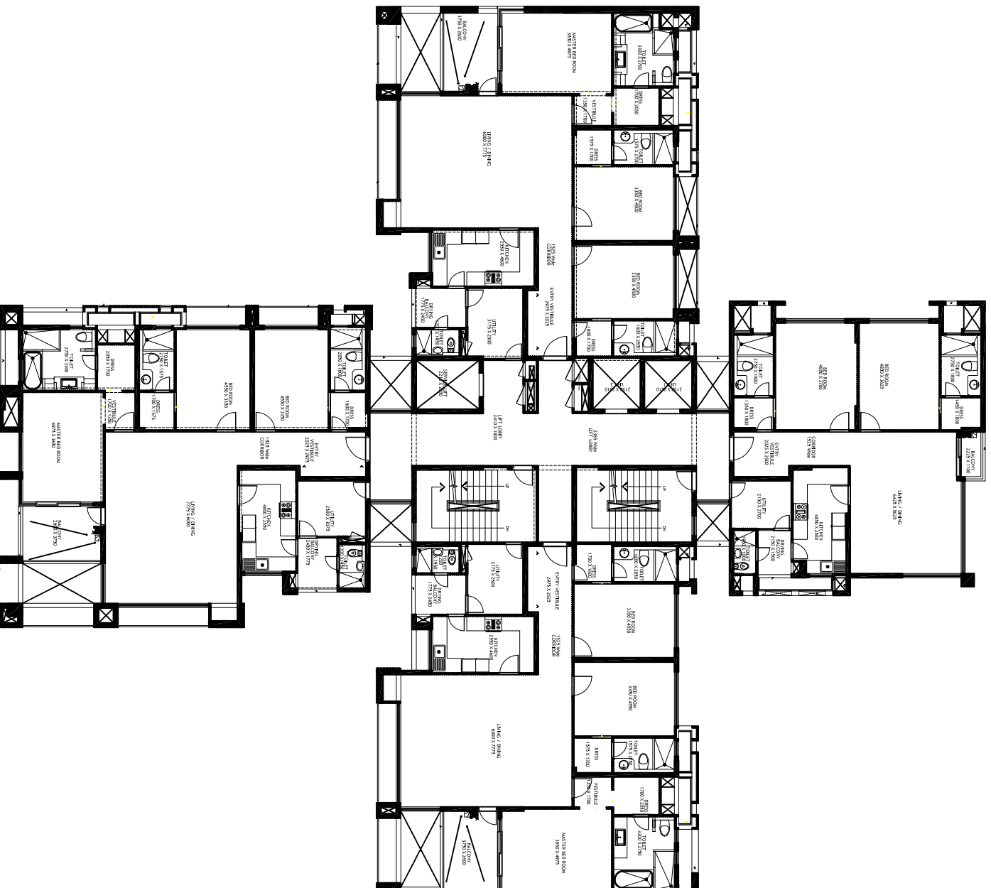
TYPICAL - 3BHK & 2BHK APARTMENTS
