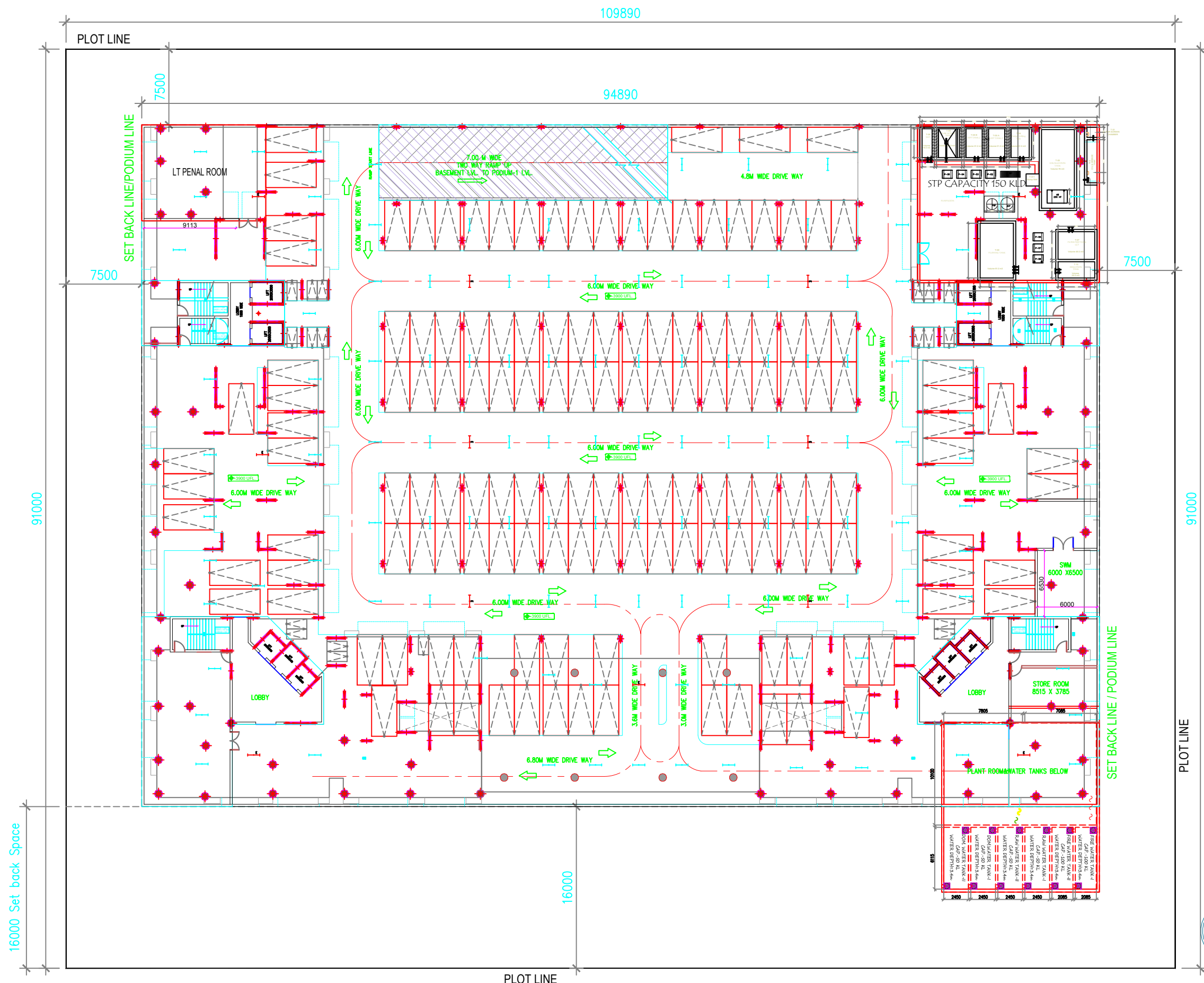
BASEMENT PLAN
