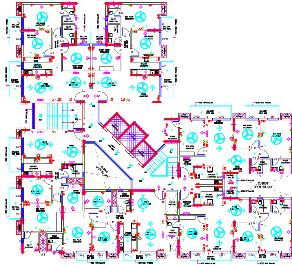
TYPICAL FLOOR ( 2ND TO 15th )PLAN OF TOWER - ( A & D )
