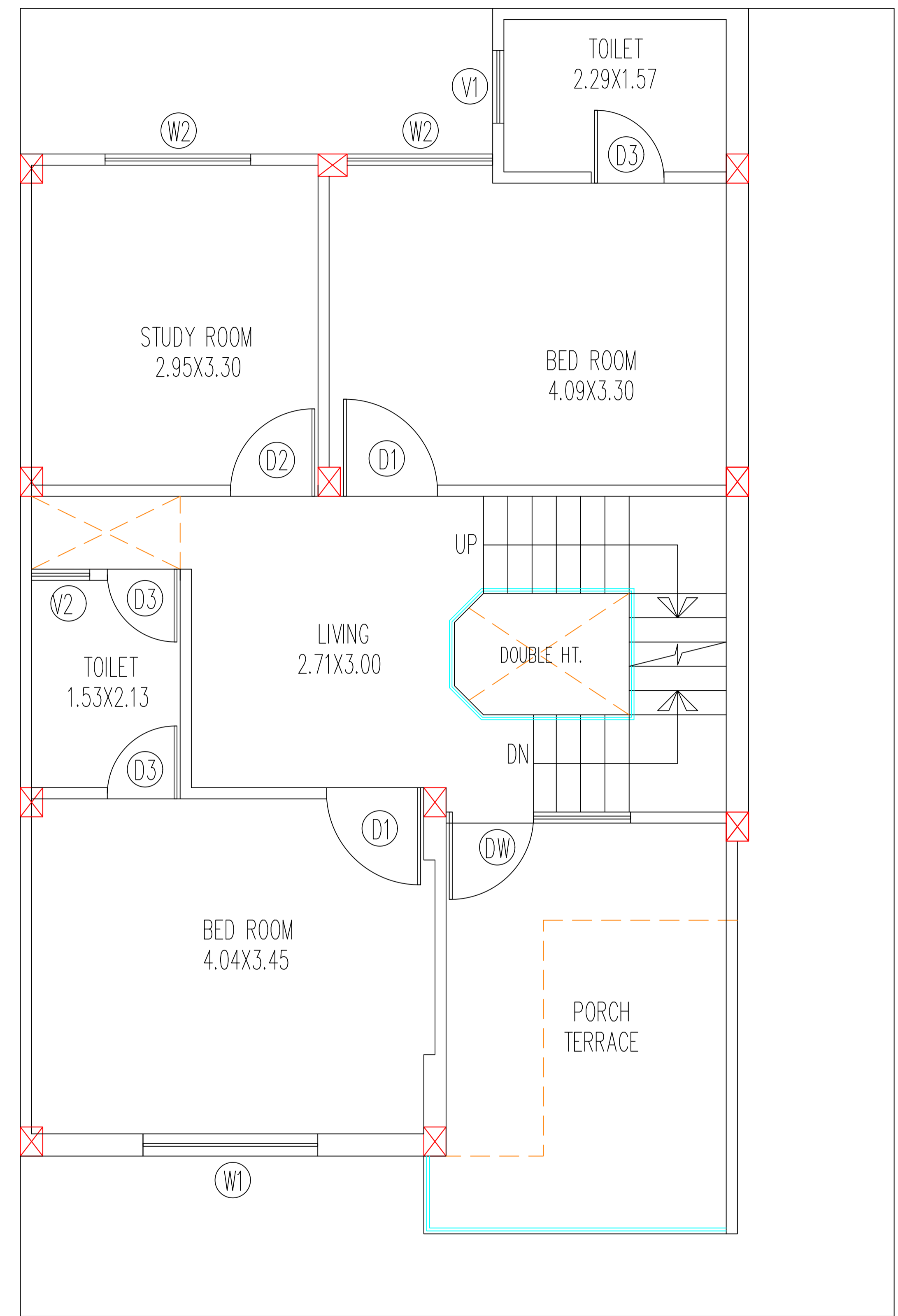
FIRST FLOOR PLAN TYPE -B
