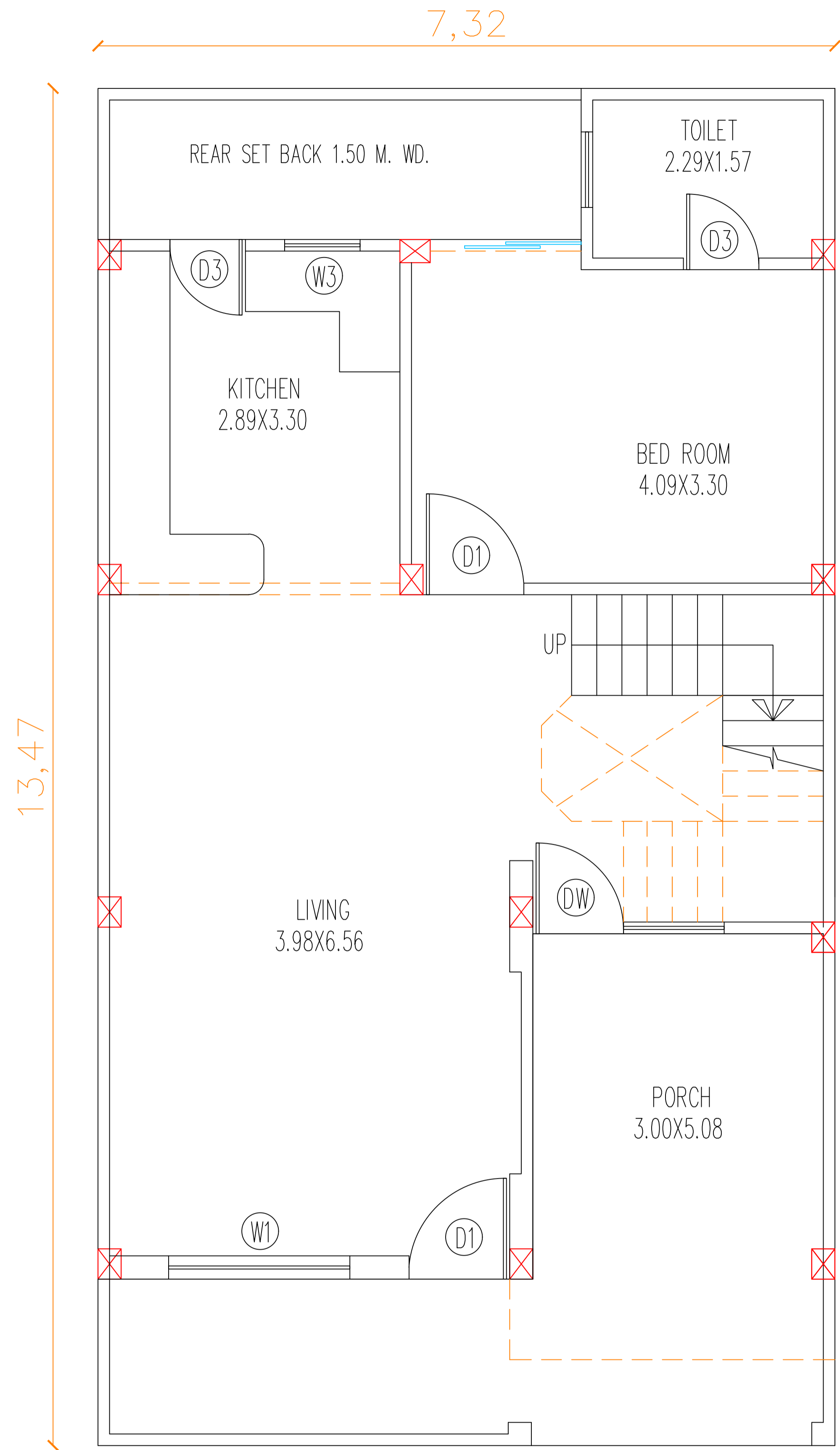
GROUND FLOOR PLAN TYPE -A
