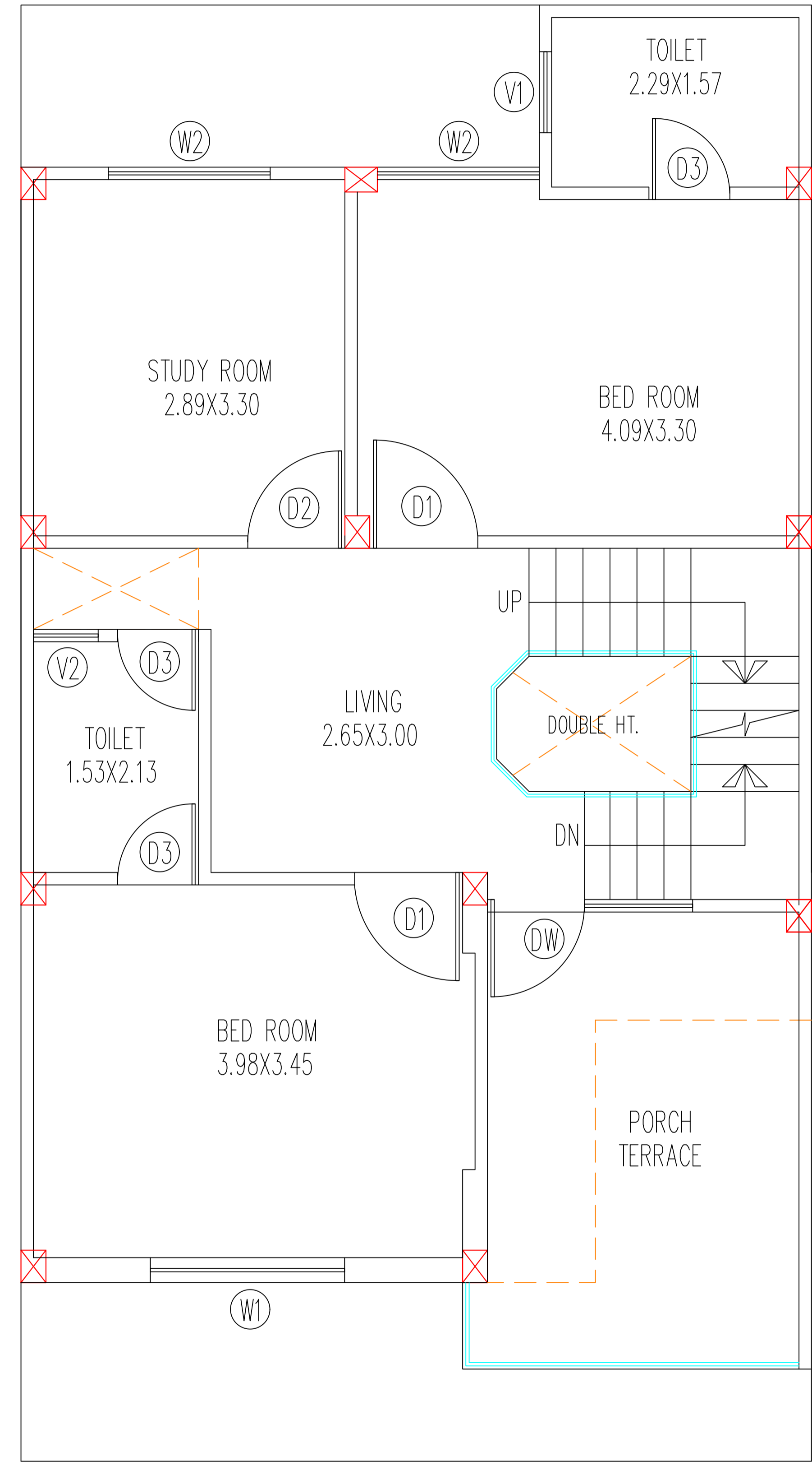
FIRST FLOOR PLAN TYPE -A
