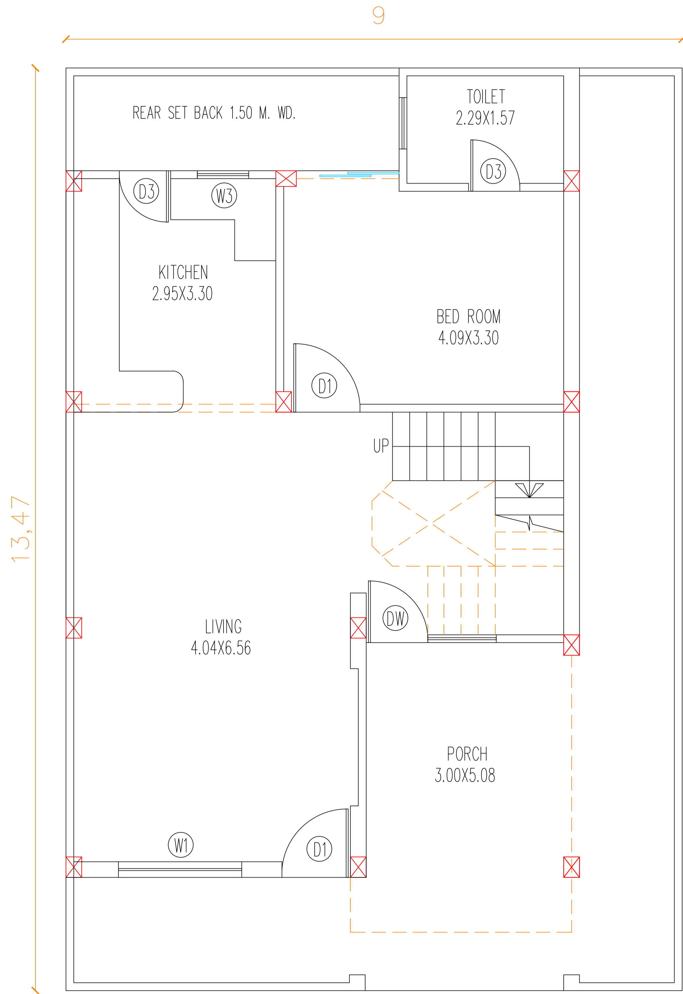
GROUND FLOOR PLAN TYPE -B
