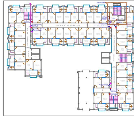
FIRST FLOOR PLAN (SCALE 1:200)
