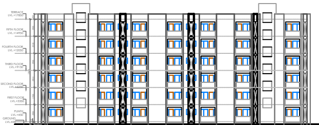
FRONT ELEVATION SCALE 1:200
