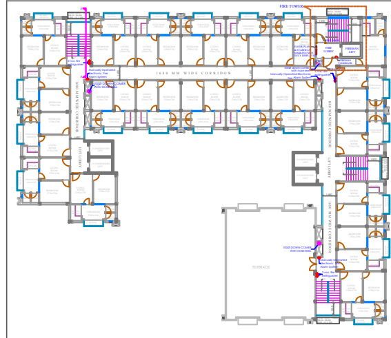
FIFTH FLOOR PLAN (SCALE 1:200)
