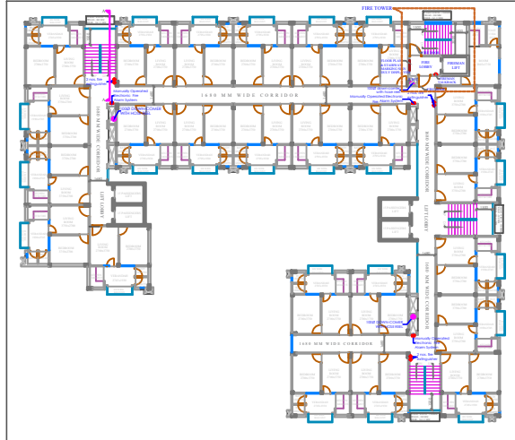
SECOND, THIRD, & FOURTH FLOOR PLAN (SCALE 1:200)
