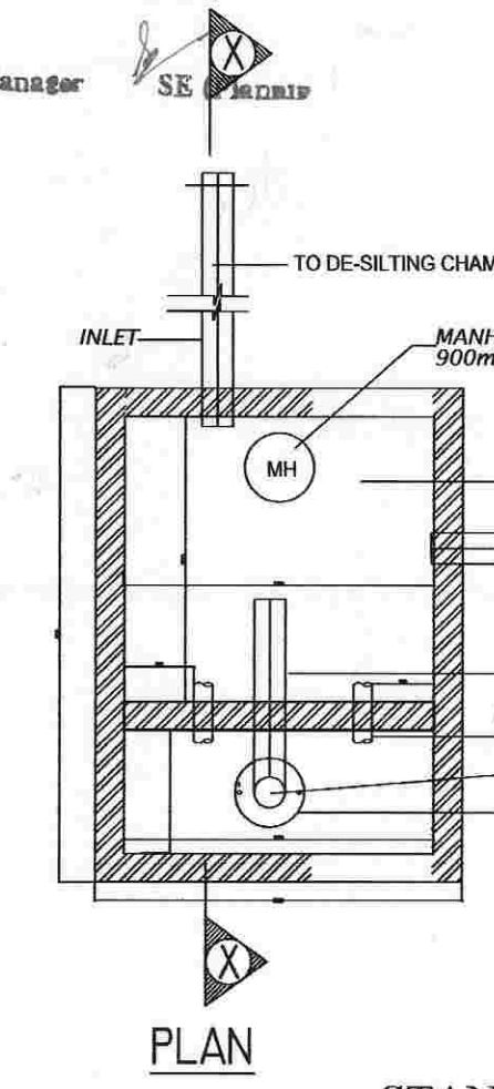
STANDARD DETAIL OF RAIN WATER HARVESTING WELL WITH DE-SILTING CHAMBER
