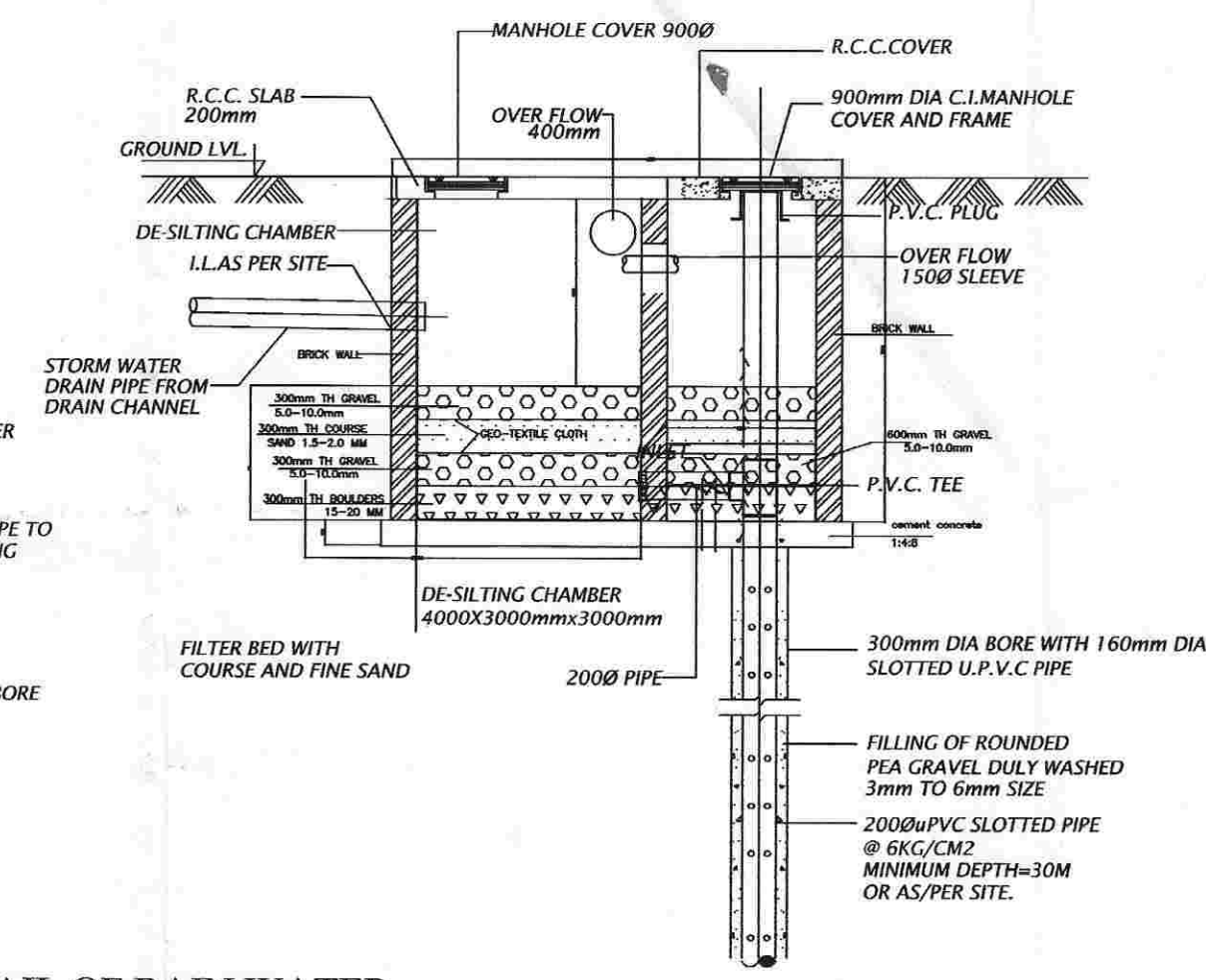
SECTION X-X
