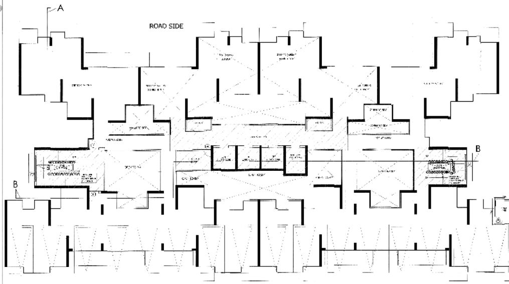
TOWER - R (B+P+27) STILT/PODIUM/GROUND LEVEL PLAN GARDEN SIDE
