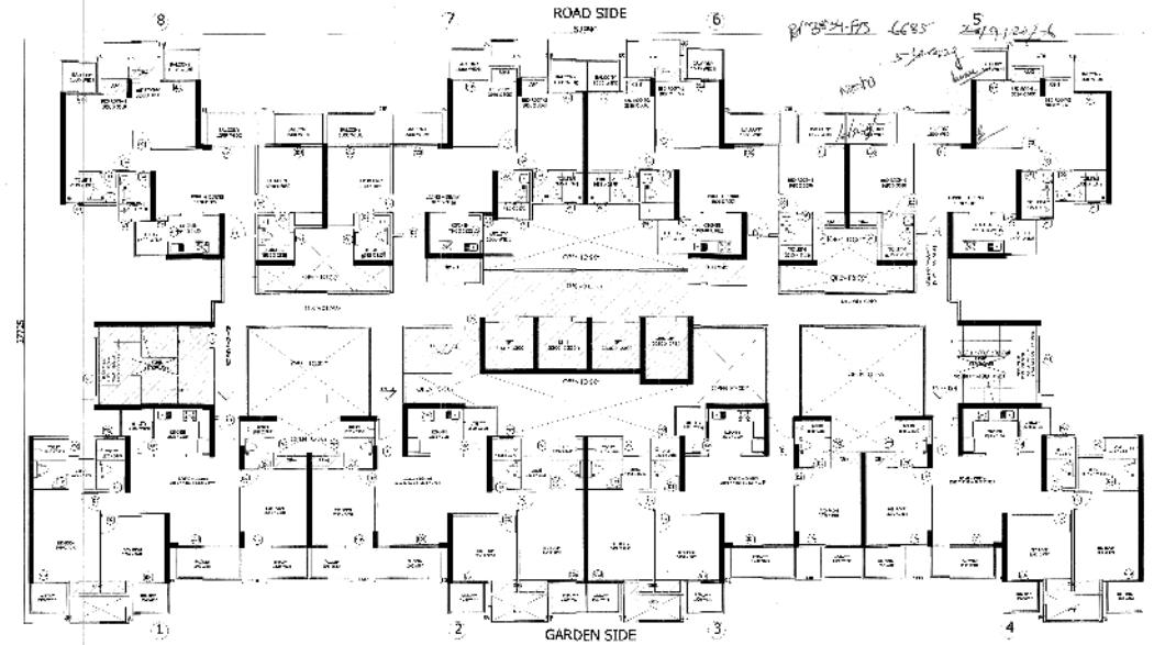
SECOND TYPICAL FLOOR 2,4,6,8,10,12,14,16,18,20,22,24 & 26 PLAN TOWER - R (B+P+27)
