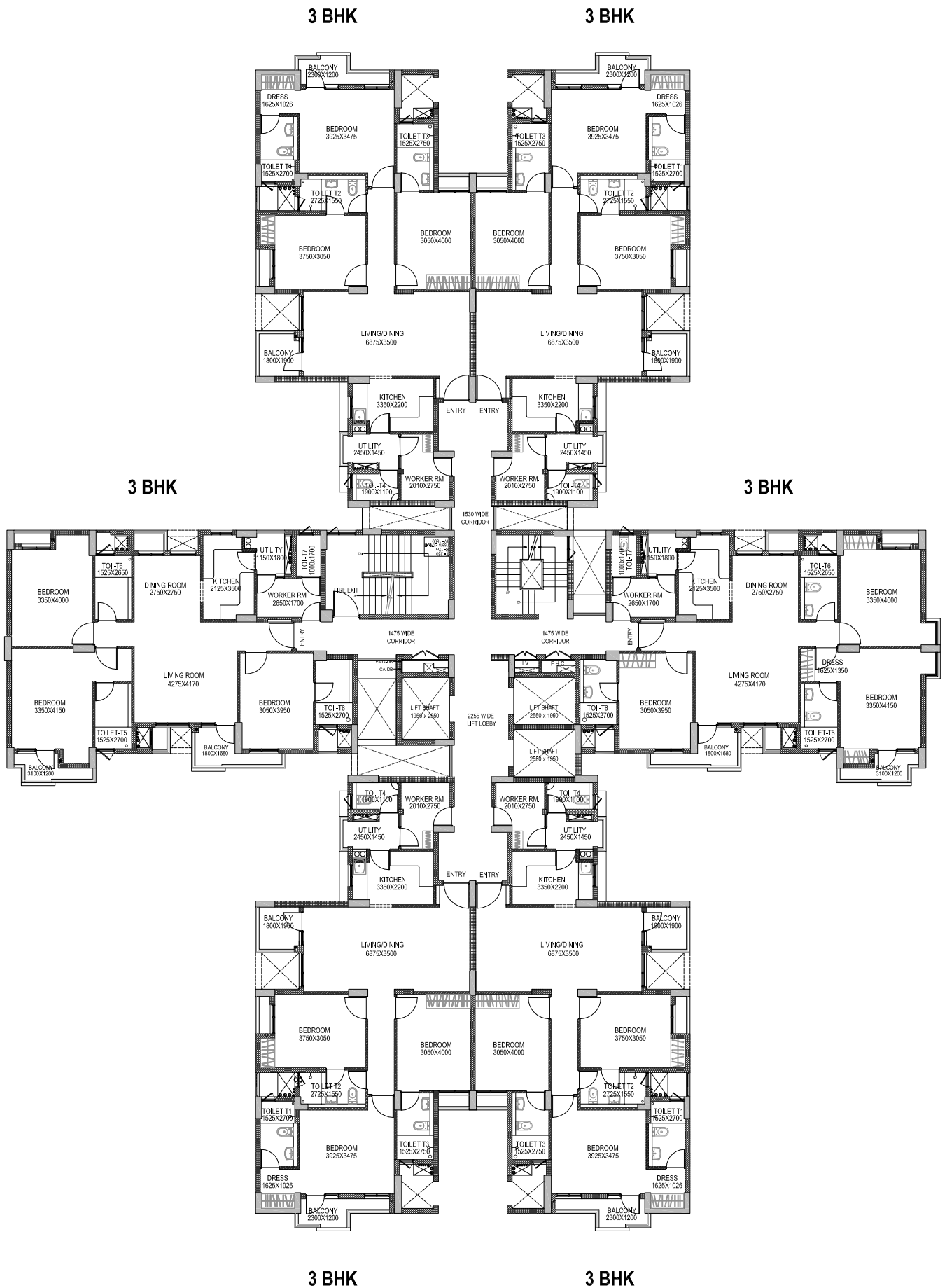
TYPE 3 TYPICAL FLOOR PLAN
