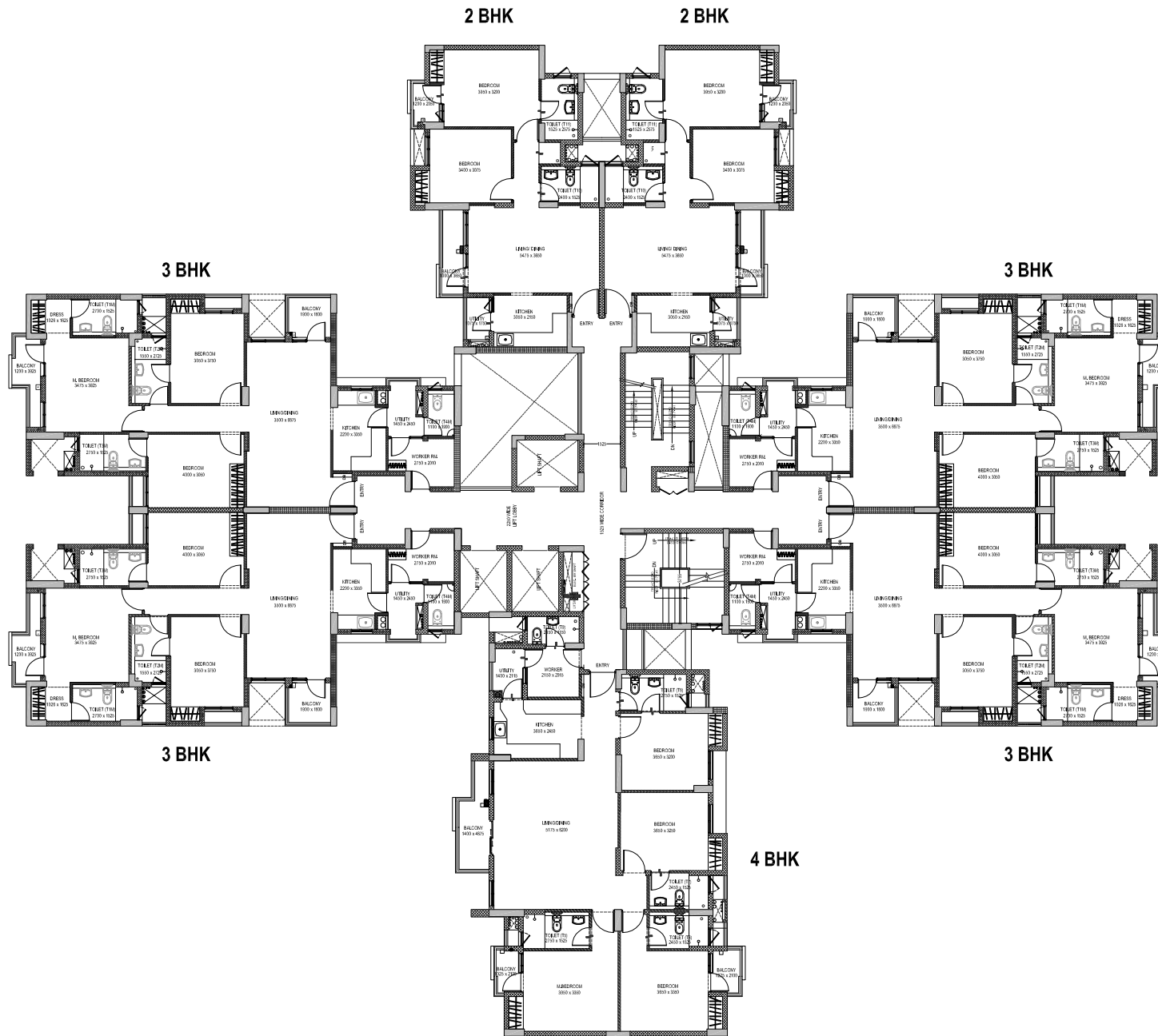
TYPE 2A TYPICAL FLOOR PLAN
