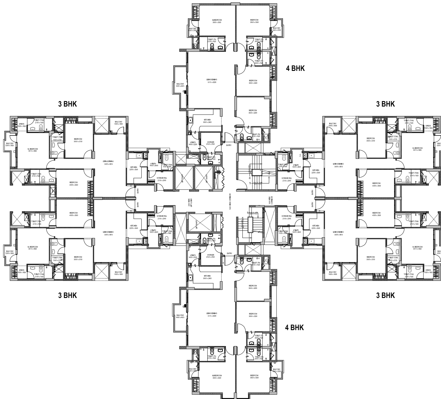
TYPE 2 TYPICAL FLOOR PLAN
