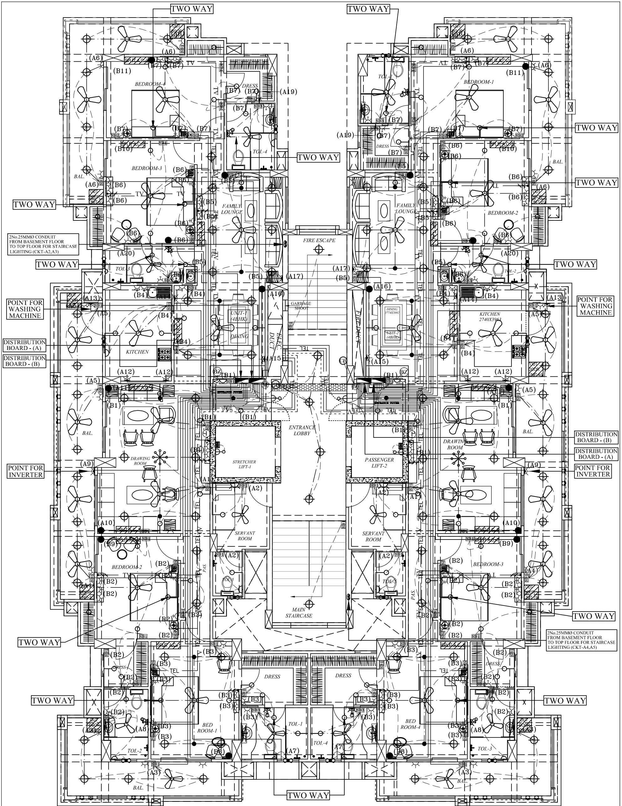
ELECTRICAL LAYOUT OF TYPICAL FLOOR
