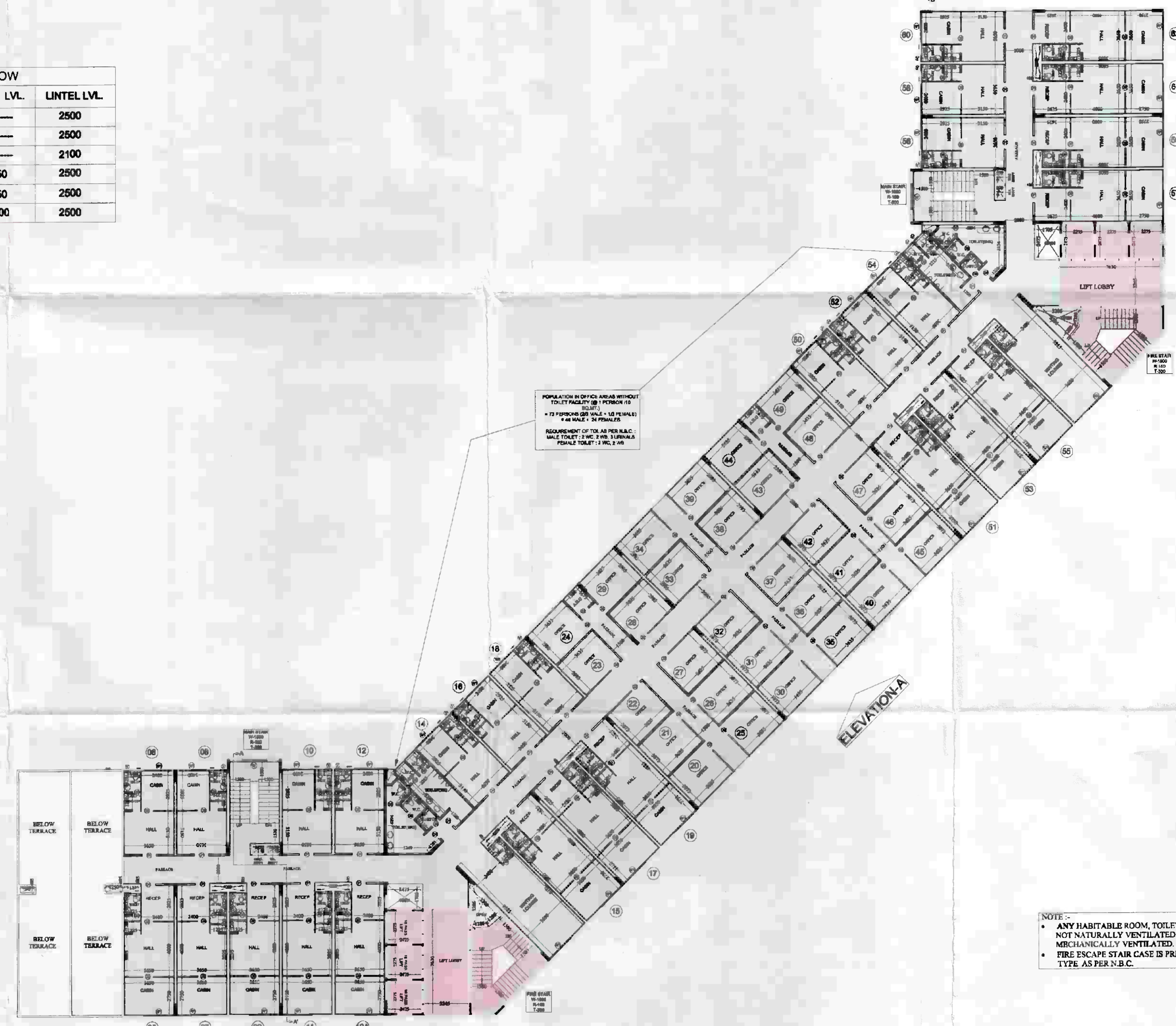
TOWER -A 8th. & 9th. FLOOR PLAN
