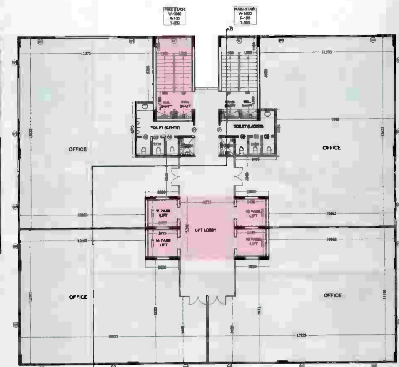
TOWER -B 5th. FLOOR PLAN
