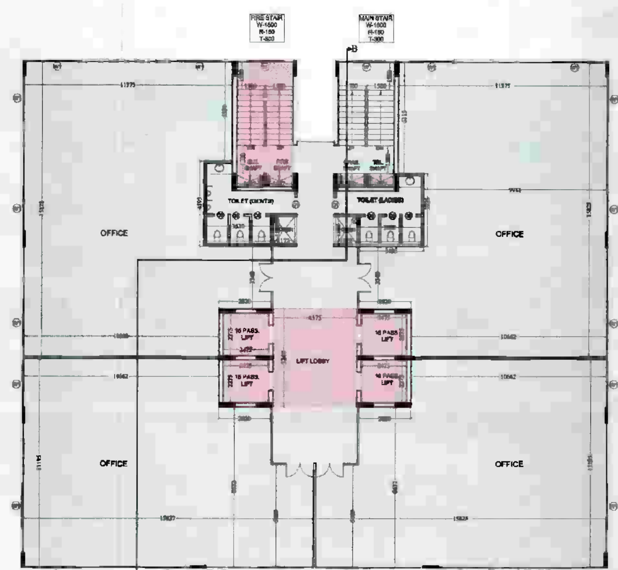
TOWER -B 11th. FLOOR PLAN
