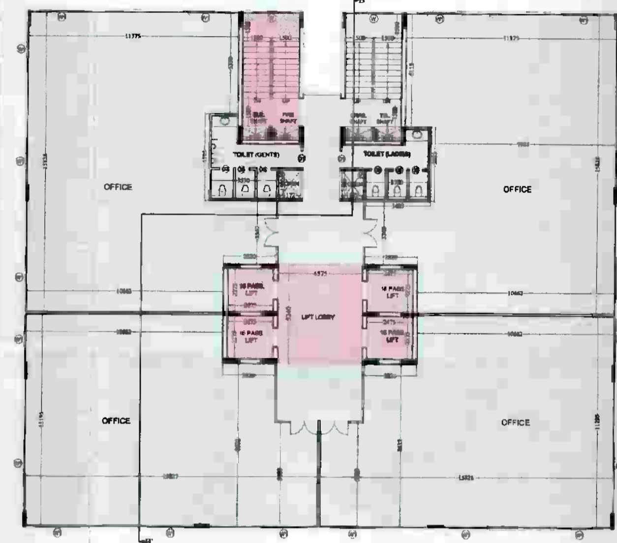
TOWER -B 7th. FLOOR PLAN
