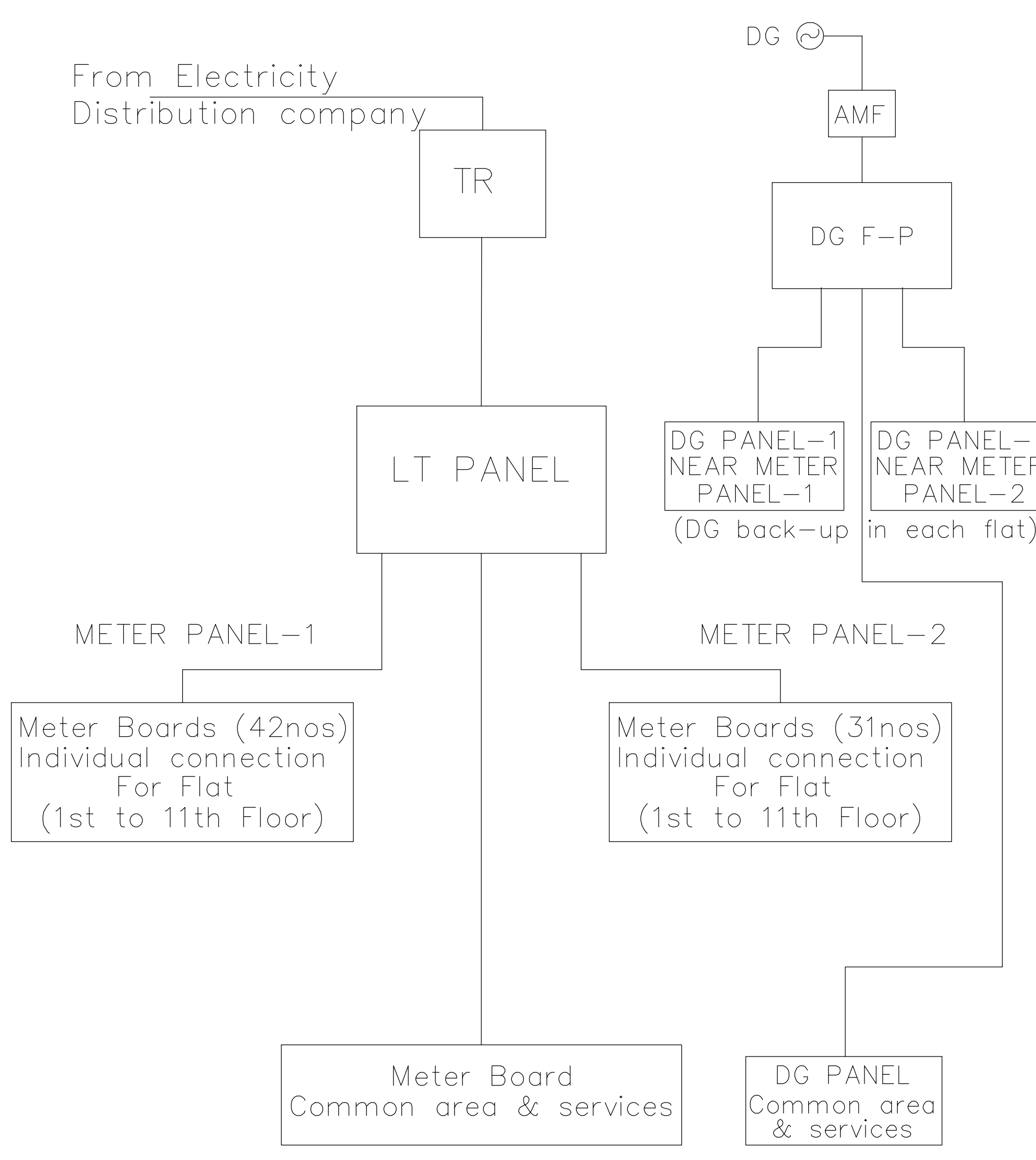
ELECTRICAL SUPPLY SCHEME
