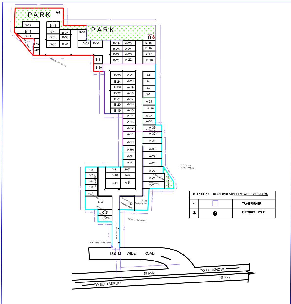
ELECTRICAL PLAN FOR VIDHI ESTATE EXTENSION
