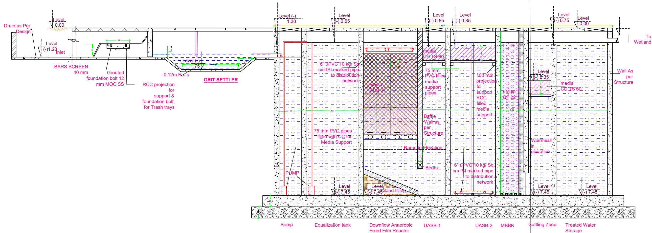
Section 1-1
