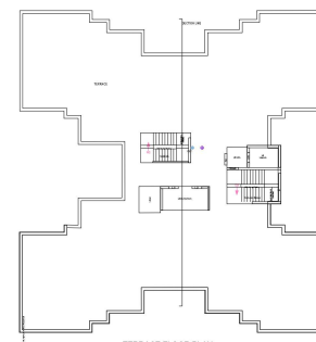
TERRACE FLOOR PLAN (SCALE 1:200) TOWER C2
